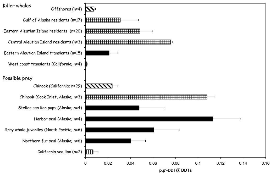
Figure 4. The ratios p,p' -DDT/ \sum DDTs \pm 1SD in adult male killer whale populations and selected putative prey species.
