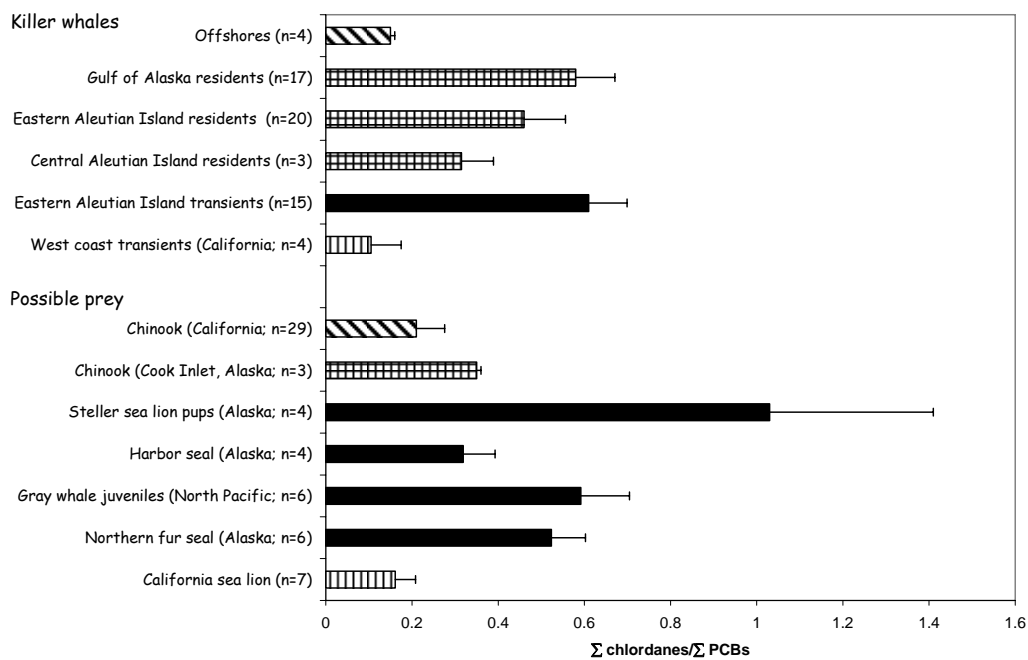
Figure 5. The ratios \sum chlordanes/ \sum PCBs \pm 1SD in adult male killer whale populations and selected putative prey species.
