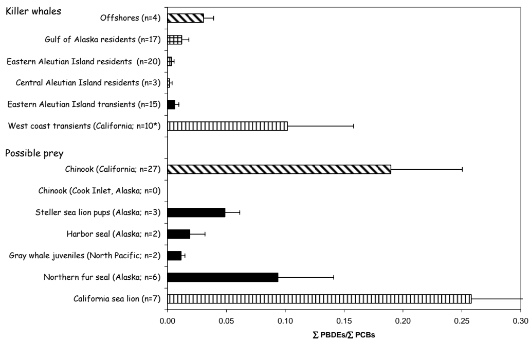
Figure 6. The ratios \Sigma PBDEs/ \Sigma PCBs \pm 1SD in adult male killer whale populations (*females were also used for West Coast transients) and selected putative prey species.
