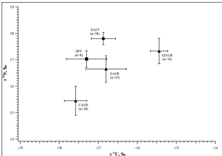
Figure 2. Nitrogen and carbon stable isotope ratios for killer whale ecotypes (T = transients; R = residents and OFF = offshores). Other abbreviations are identical to those reported in Figure 1.
