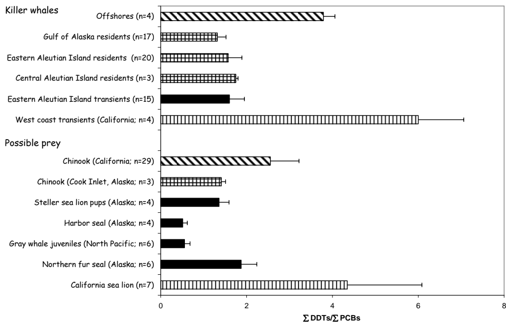
Figure 3. The ratios \Sigma\text{DDTs}/\Sigma\text{PCBs} \pm 1\text{SD} in adult male killer whale populations and selected putative prey species (matching patterns).
