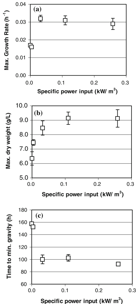
Fig. 3 Relationship between specific power input (kW/m 3 ) and growth rate (a); maximum dry cell weight (b); and fermentation rate (c). Error bars, SE of mean of at least two experiments
