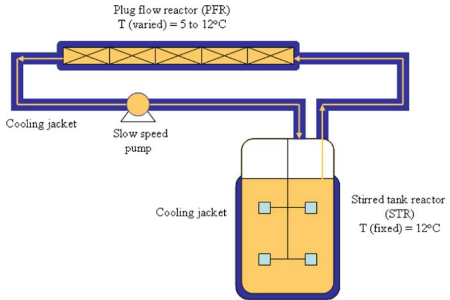
Fig. 5 Schematic of scale-down model to simulate temperature variations in an industrial scale brewer fermenter
