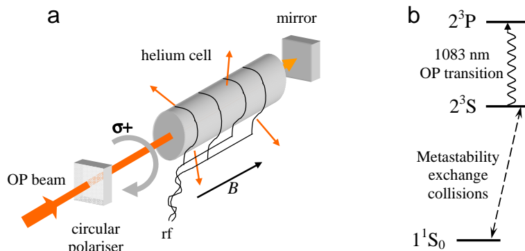
Figure 1. a: Schematic view of a basic MEOP set-up. In a {}^3\text{He} gas cell, a weak rf discharge promotes a small fraction of the atoms into the excited metastable state 2^3\text{S} , where resonant absorption of 1083 nm light occurs. This OP light is circularly polarised and propagates along the direction of the applied magnetic field B . For enhanced absorption, the light is usually back-reflected for a second pass through the cell. Nuclear polarisation is transferred to atoms in the ground state by metastability exchange collisions. b: The atomic levels of He and the main physical processes involved in MEOP are shown. The 2^3\text{S} and 2^3\text{P} states are composed of several levels and the 1083 nm line thus has a complex structure (see Fig. 2).
