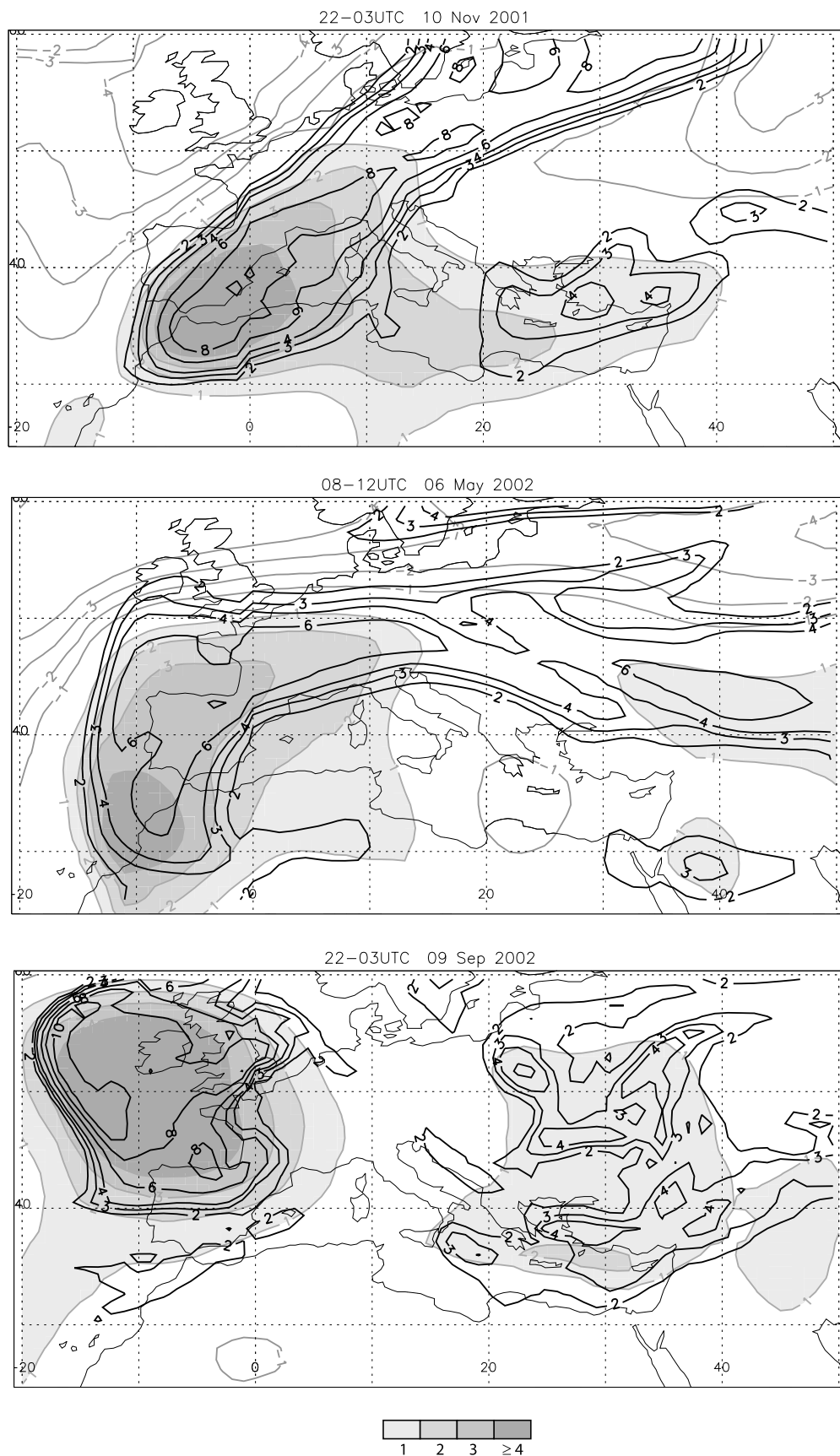
Figure 3. Winter and transition months cases: A8 BT anomaly (BT', in K) relative to a monthly mean of 2001–2006 (shaded > 1 K, gray contours < -1 K) and PV at 250 hPa (PVU, 1 PVU = 10^{-6} \text{ K m}^2 \text{ kg}^{-1} \text{ s}^{-1} ; black contours) for the dates indicated on the top of each panel.
