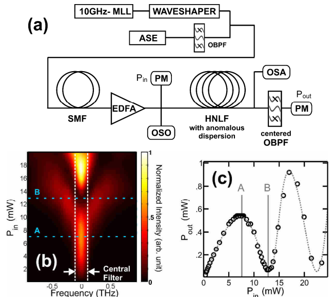
Fig. 1: (a) Experimental set-up. PM : powermeter (b) Evolution of the experimental optical spectrum recorded after the HNLFF as a function of input average power. Dashed white line illustrates the FWHM of the OBPF. (c) Transfer function of the device: experimental results (circles) are compared with numerical simulations (dashed grey line).
