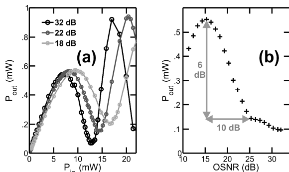
Fig. 4: (a) Influence of the OSNR on the TF. (b) Output average power as a function of the input signal OSNR for a working power of 12.9 mW.
