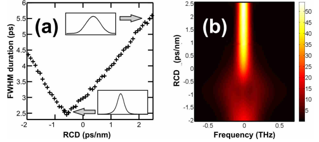
Fig. 2: (a) FWHM temporal duration of the pulse entering the HNLf according to the RCD induced by the dispersion emulator. Insets : temporal intensity profiles recorded over a time span of 15 ps. (b) Experimental demonstration of the influence of the RCD on the resulting spectrum recorded at the output of the HNLf and for a working average power of 7.25 mW.
