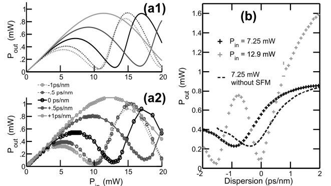
Fig. 3: (a) TF for various amounts of RCD. Numerical simulations (a1) are compared with experimental results (a2). (b) Influence of the RCD on the output power for two WPs : initial average power of 7.25 mW (black crosses) and 12.9 mW (grey crosses). The results without the SMF (numerical simulations) are plotted using a dashed black line.
