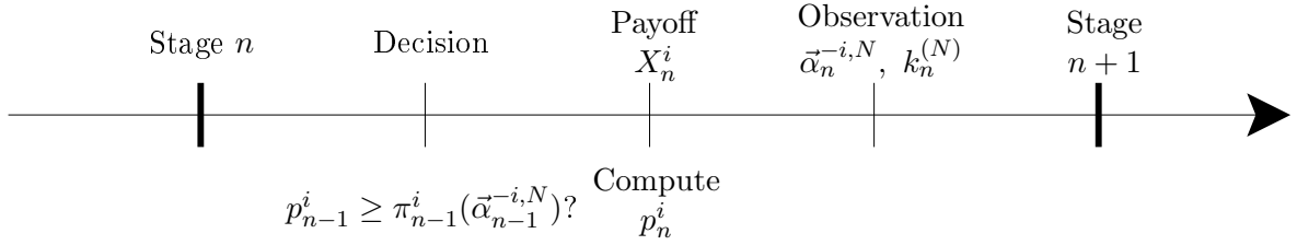
Figure 1: Progress of the game in cutoff strategy.
