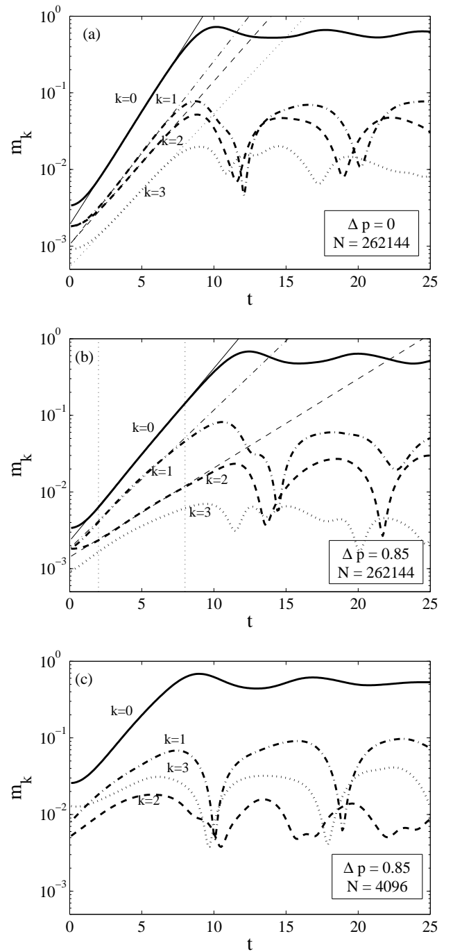
Figure 1: Time evolution of the Fourier modes of the magnetization m_k(t) (44) for the \alpha -HMF model. The initial waterbag distribution is uniform in q \in [0, 2\pi] and in p \in [-\Delta p, \Delta p] with \Delta p = 0 in panel (a) and \Delta p = 0.85 in panels (b) and (c). For these values of \Delta p the homogeneous waterbag is unstable. The Fourier modes m_k are plotted vs. time for k = 0 (thick full line), k = 1 (thick dash-dotted line), k = 2 (thick dashed line) and k = 3 (thick dotted line). The thin lines are exponential fits. The two upper panels have N = 2^{18} , while the lower panel has N = 2^{12} and shows the strong finite-size effects: the exponential growth is no more clearly visible.
