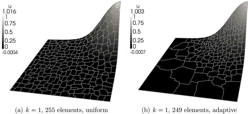
Figure 13: BRMPS solution for the test case of Karniadakis and Sherwin [16].
