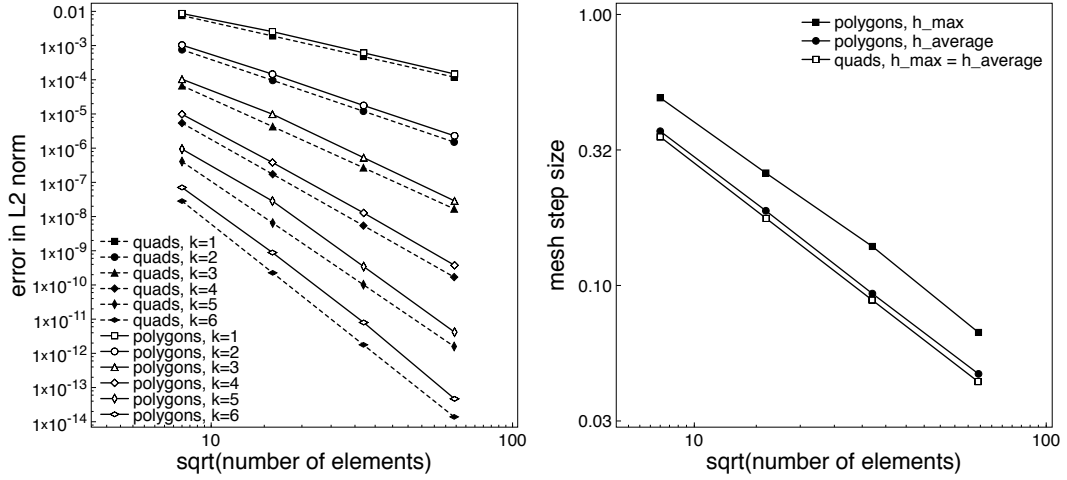
Figure 8: Left. Convergence of the L^2 -orthogonal projection on uniform quadrilateral grids (solid lines) and polygonal grids obtained by agglomeration (dashed lines), k \in \{1, \dots, 6\} . Right. Maximum and average mesh size h on uniform grids and polygonal grids.
