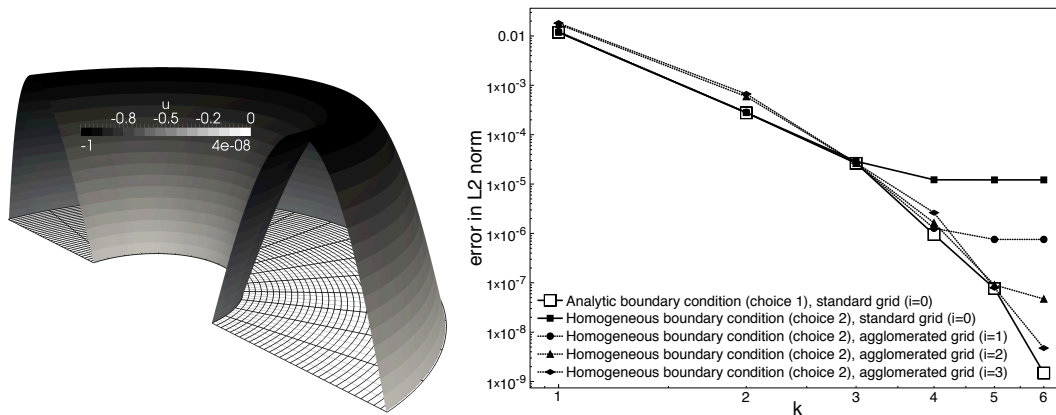
Figure 10: Test case proposed by Gobbert and Yang [14]. Left , Solution on a 32 \times 32 grid (thick lines) agglomerated on top of a 128 \times 32 quadratic quadrilateral mesh (thin lines), k = 6 approximation (half of the domain is sketched). Right , k -convergence of the BRMPS discretization using a 32 \times 32 agglomerated grid and various underlying fine meshes and boundary conditions, see text for details.
