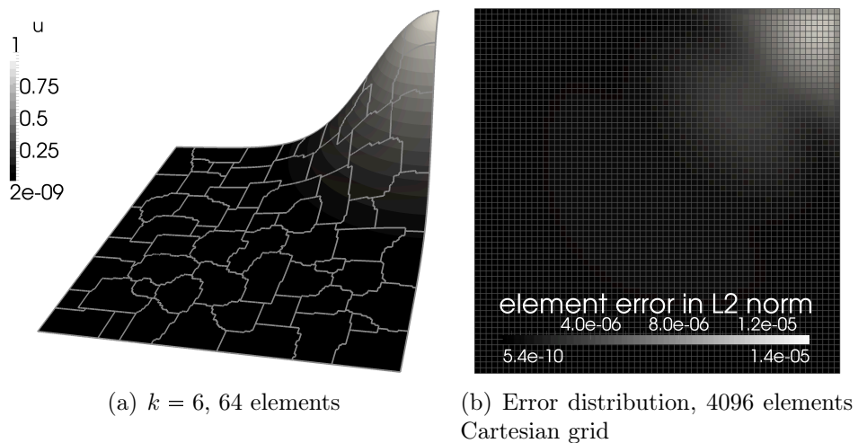
Figure 7: BRMPS solution for the test case of Karniadakis and Sherwin [16].
