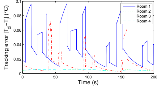
FIG. 6. Temperature tracking error without communication constraints
