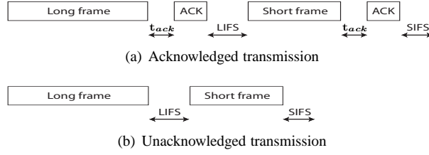
FIG. 3. IFS data transmission mechanism with and without acknowledgement.
