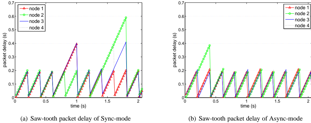
FIG. 5. Saw-tooth packet delay with 70 bytes packets and four nodes for two traffic generation models.
