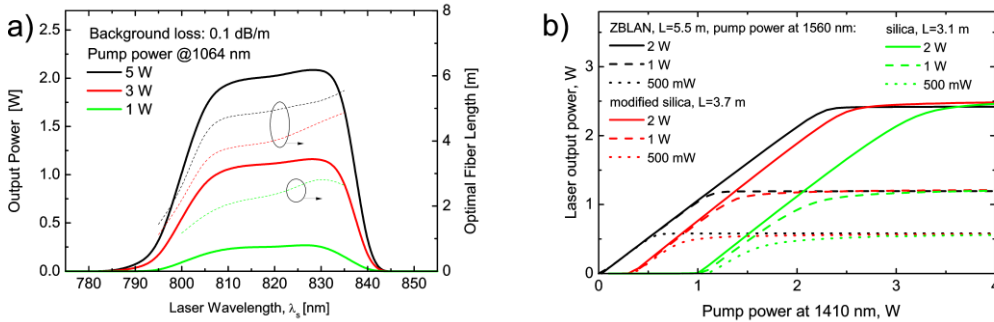
Fig. 6. (a) Laser wavelength tuning characteristics. (b) Examples of the dual-wavelength pumped upconversion laser. The output power at 810 nm is plotted vs. the pump power at 1410 nm (ESA {}^3F_4 \rightarrow {}^3H_4 ) for the three different host materials and for three pump power levels at 1560 nm (ground state absorption {}^3H_6 \rightarrow {}^3F_4 ).
