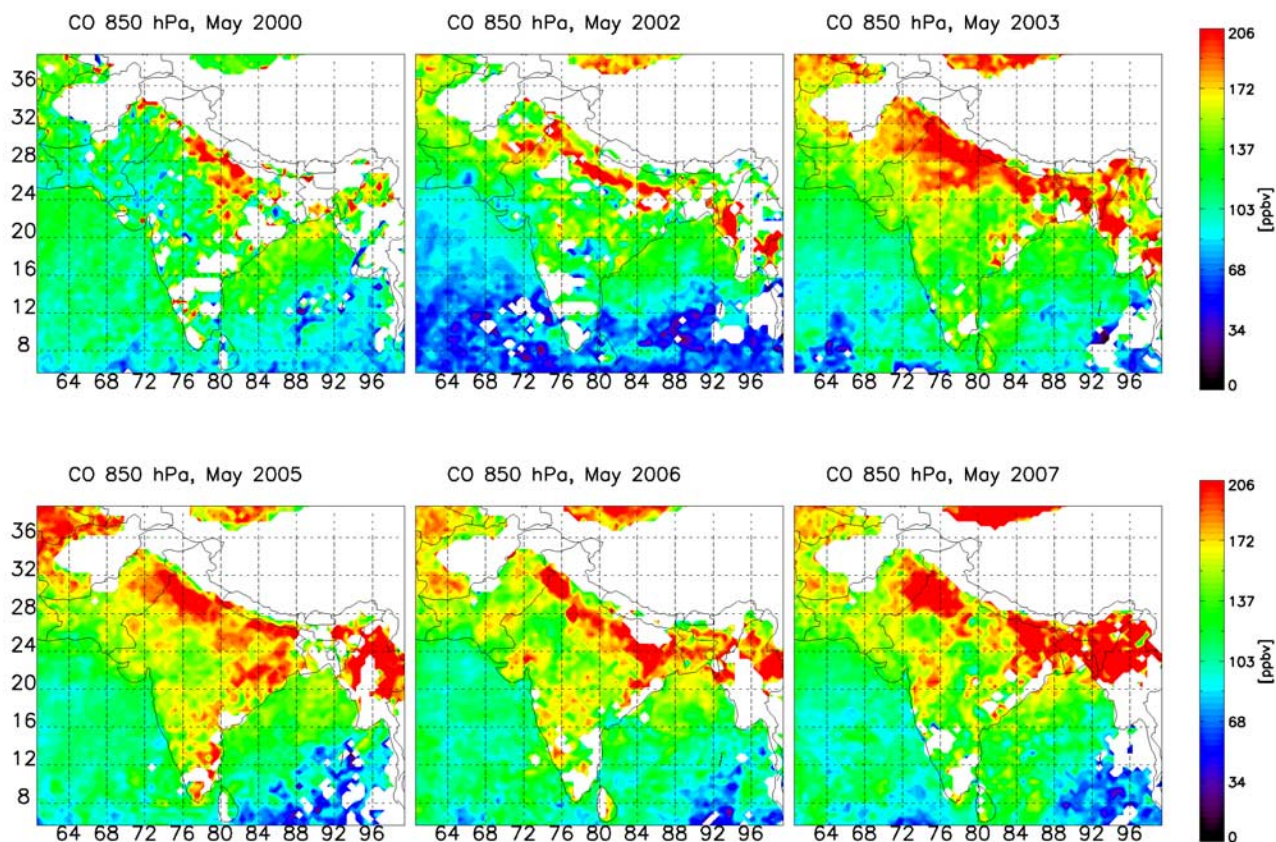
Figure 7a. CO mixing ratio (ppbv) retrieved at 850 hPa level by MOPITT over the Indian subcontinent for May 2000, 2002, 2003, 2005, 2006, and 2007. Data binned in 0.5^\circ in latitude and longitude, and white areas indicate missing data. Only daytime data have been used. Data for May 2001 are not available.
