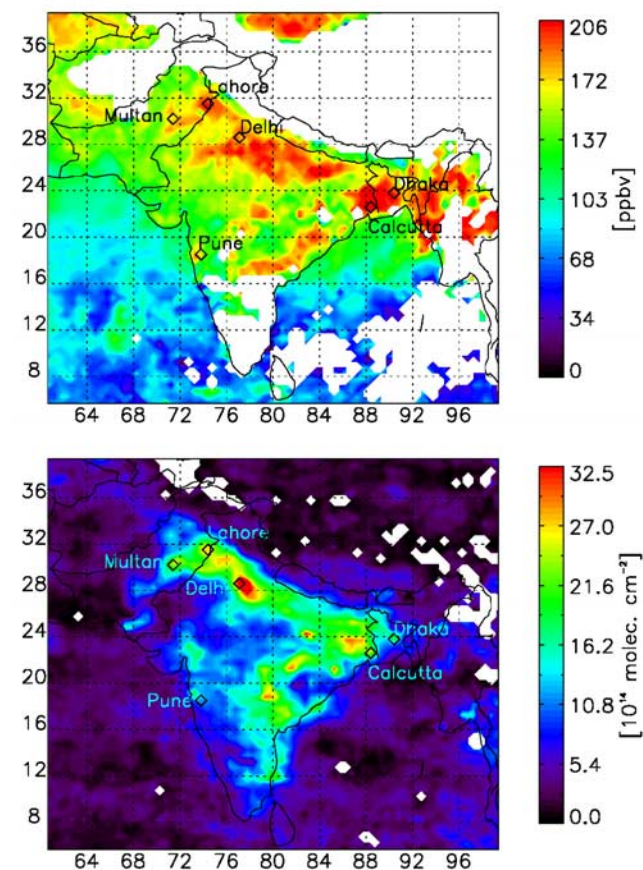
Figure 2. Distribution of MOPITT CO mixing ratios (ppbv) at 850 hPa (top) and SCIAMACHY tropospheric column \text{NO}_2 ( 10^{14} \text{cm}^{-2} ; bottom). Data have been binned in 0.5^\circ in latitude and longitude. Both distributions are for May 2004. Only daytime data from MOPITT measurements have been used. The white areas indicate data dropouts due to clouds or topography. Locations of some of the cities with large population are marked out.
