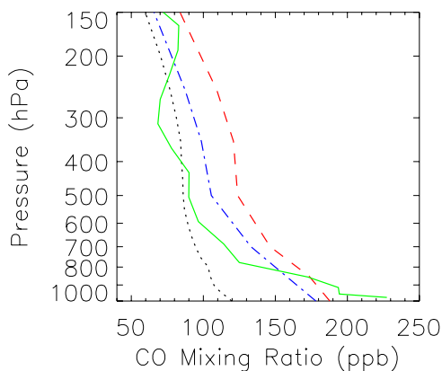
Figure 6. Comparison of MOPITT and GEOS-Chem profiles of CO on 29 May 2004 at 87°E, 24°N. The MOPITT profiles have been averaged on the GEOS-Chem 2^\circ \times 2.5^\circ grid. The retrieved MOPITT profile and the a priori profile used in the retrieval are shown as the red dashed and black dotted lines, respectively. The GEOS-Chem profile of CO is shown as the green solid line, whereas the modeled profile transformed by the MOPITT averaging kernels and a priori profile is indicated by the blue dash-dotted line.
