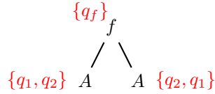
Figure 3. A run of \mathcal{A}^{(2)} on f(A, A) .
