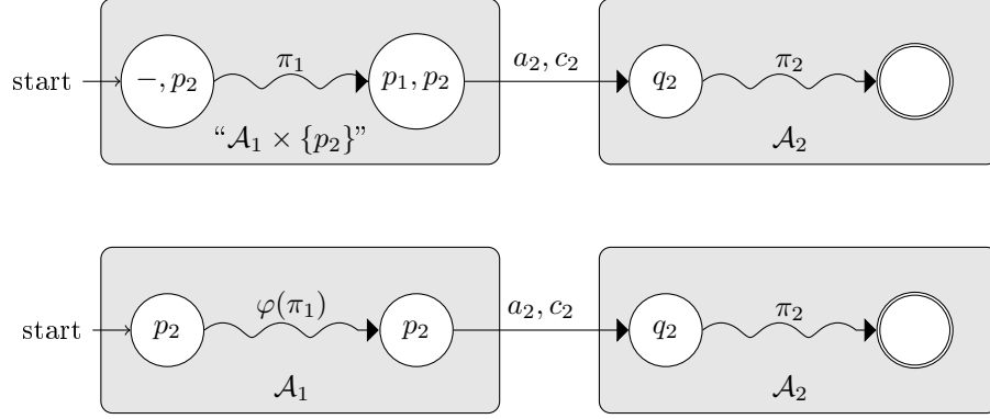
Figure 7: Proof of Proposition 11.
