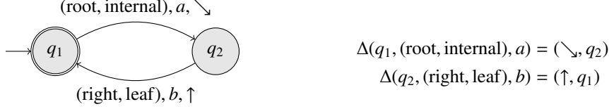
Figure 2: A deterministic tree walking automaton.
