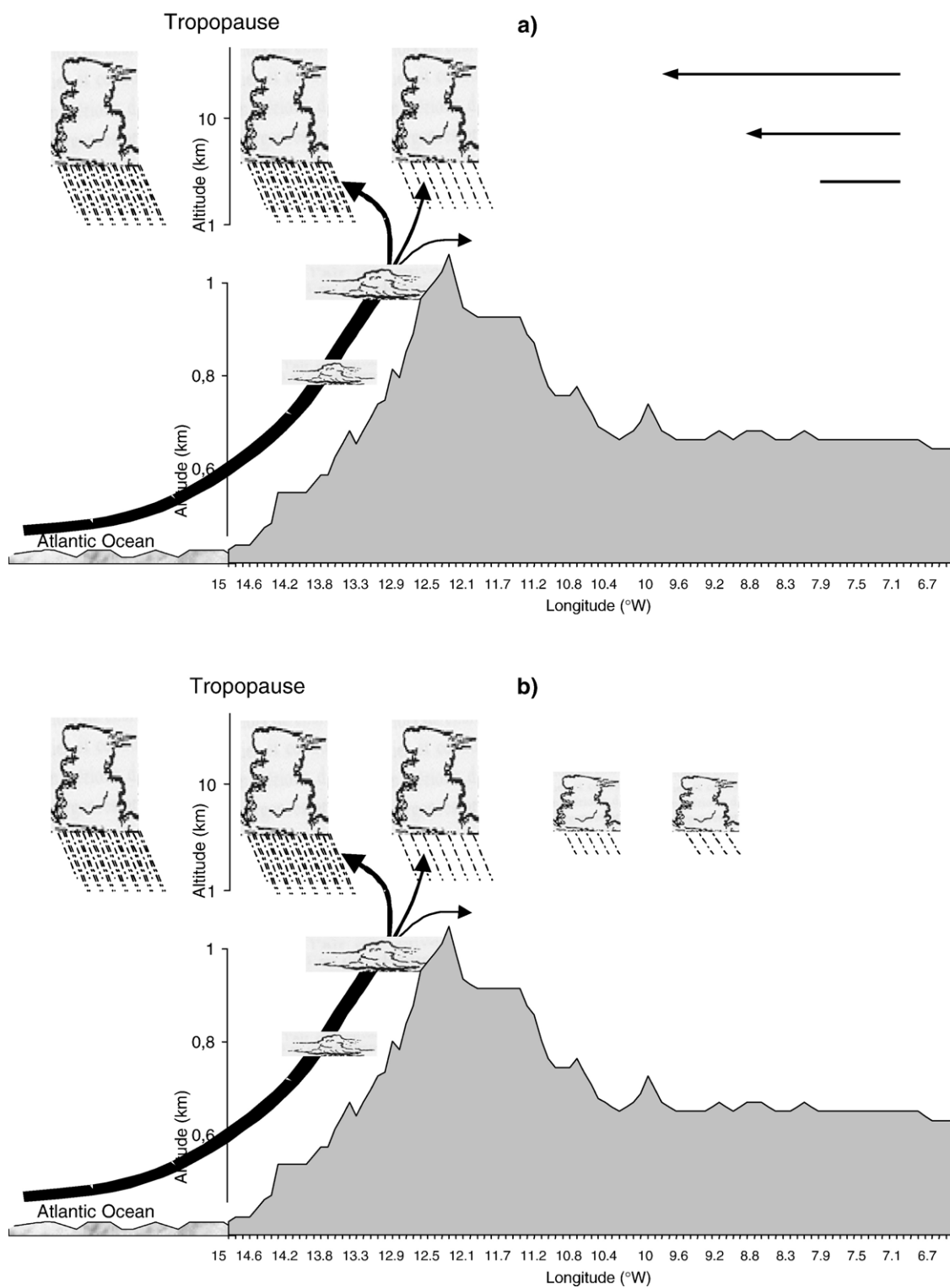
Fig. 16. Conceptual scheme of convection development over the relief of the Fouta Djallon (see text). a) Case of local convection; b) Case of drifting MCSs.
