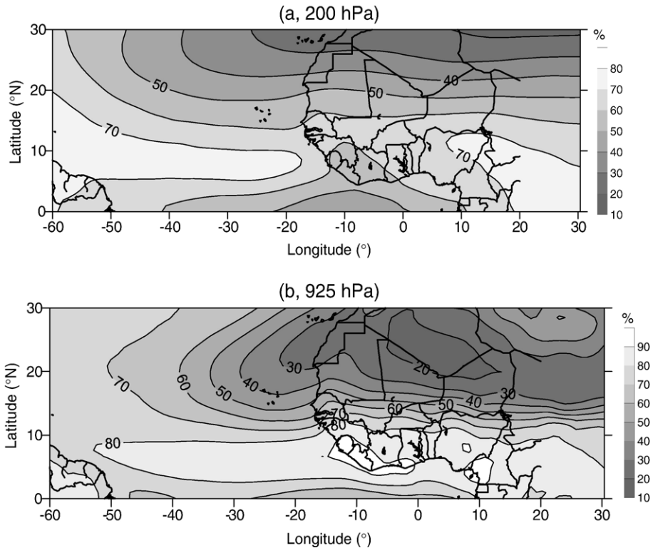
Fig. 6. Relative humidity averaged over 23 years (1979–2001) at a) 200 hPa and b) 925 hPa. Isolines are in percent (from reanalyses of ERA 40).
