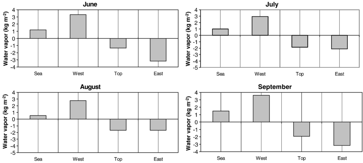
Fig. 12. Differences between the monthly average of vertically integrated water vapor content in the zone ( 5^{\circ}\text{N} – 15^{\circ}\text{N} ), ( 2.5^{\circ}\text{W} – 20^{\circ}\text{W} ) averaged from 1989 to 1998 and monthly average over the same period observed in the four areas of Fig. 1 for the months of the rainy season (from reanalyses of ERA 40).
