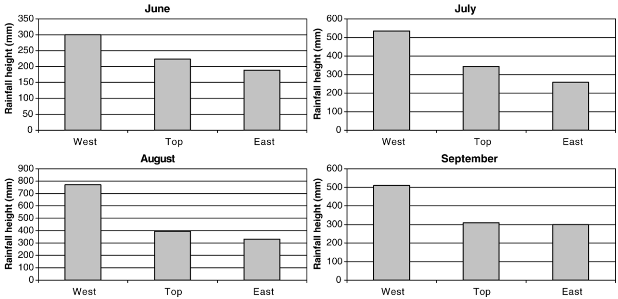
Fig. 15. Distribution of monthly rainfall height averaged from 1925 to 1975 for JJAS (from data of Nicholson et al. 1988).
