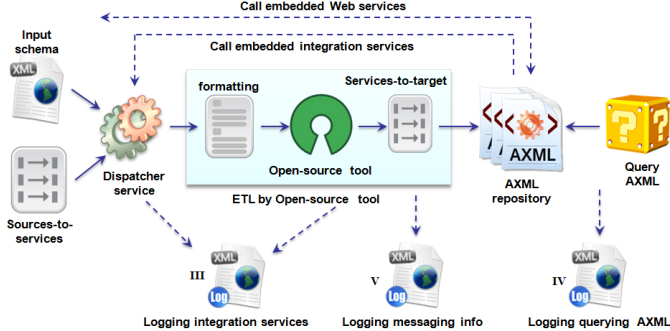
Fig. 6. Integrating complex data using open-source tool workflow
