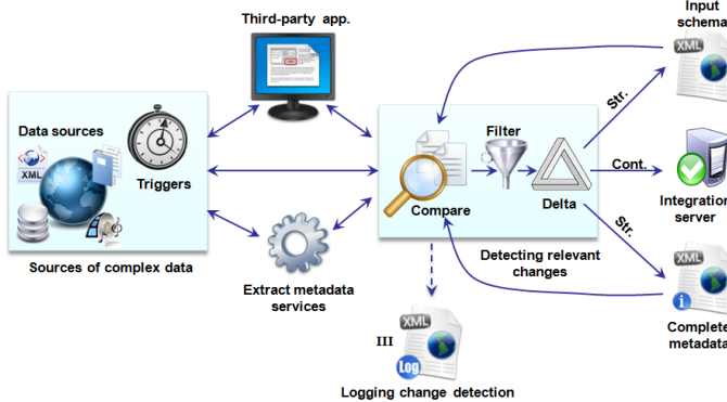
Fig. 5. Monitoring change detection workflow
