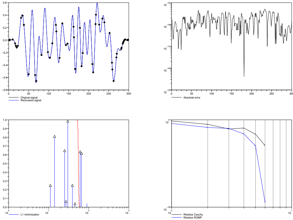
Fig. 7. Exact recovery of \vec{f} with \|\vec{f}\|_{\ell^0} = 9 from 61 samples taken as random.
