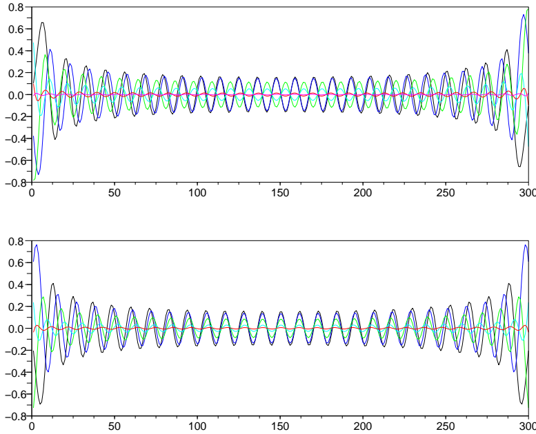
Fig. 4. Delocalized PSWF with k \simeq 2c/\pi and c = 85 (top: odd, bottom: even).
