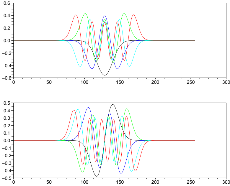
Fig. 1. First 10 PSWF (top: even, bottom: odd) with c = 130 and T = 1 .
