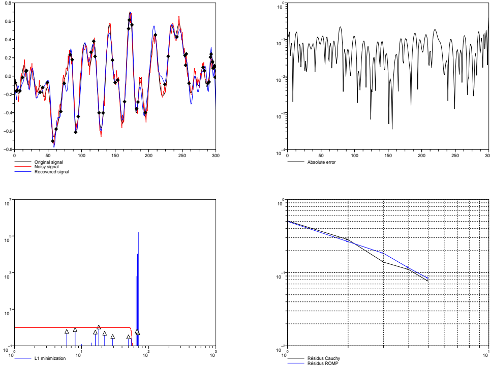
Fig. 9. Recovery with 10% of noise, s = 9 , c = 85 and N = 15 + \frac{2c}{\pi} .
