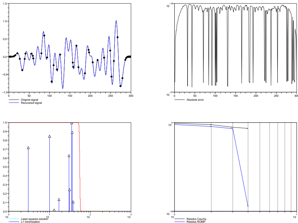
Fig. 6. Exact recovery of \vec{f} with \|\vec{f}\|_{\ell^0} = 9 from 54 samples taken as random.
