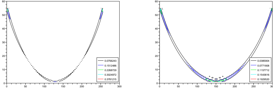
Fig. 5. Biggest values appearing in the PSWF sensing 256 \times 55 matrix (left, used in §3) and in the preconditioned 300 \times 55 one (right).
