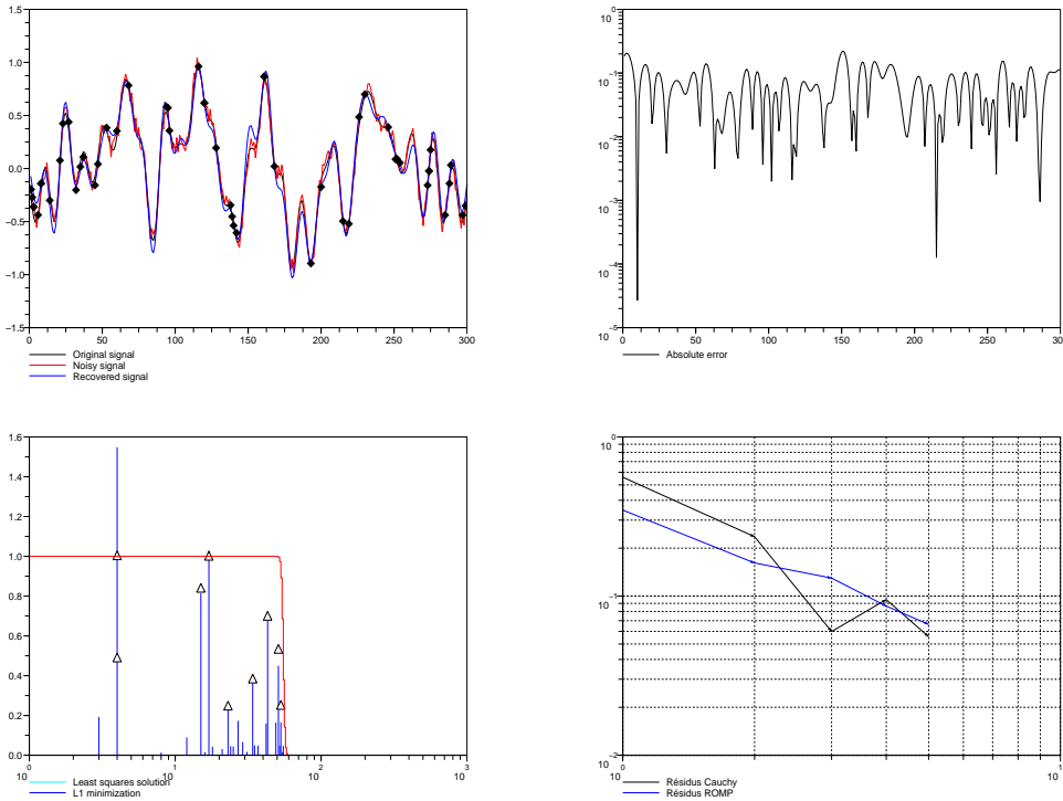
Fig. 8. Recovery involving 10% of noise with s = 9 and c = 85 .
