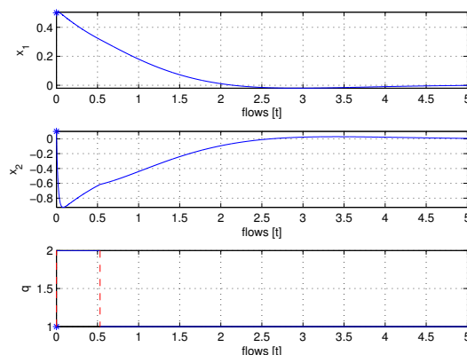
Fig. 1. At top, time evolution of x_1 , at middle, time evolution of x_2 and, at bottom, time evolution of q .
