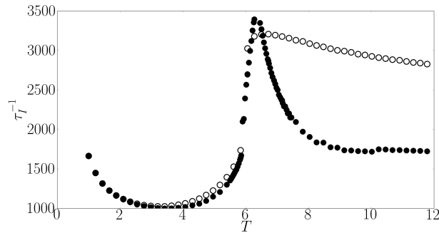
FIG. 4: BCC ferromagnetic film: Inverse of relaxation time of itinerant spins \tau_I^{-1} calculated with temperature-independent (white circles) and temperature-dependent (black circles) of the lattice spins versus temperature T , in zero magnetic field, with electric field \epsilon = 1 , I_0 = 2 , K_0 = 0.5 .
