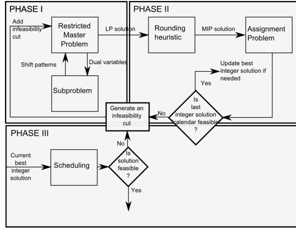
Figure 2: Scheme of the decomposition algorithm
