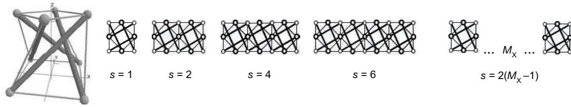
Figure 4. Number of selfstress states in a quadruplex beam.
