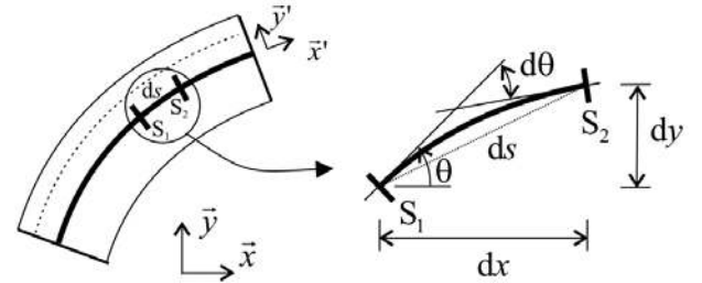
Figure 10. Relative rotation of two sections
