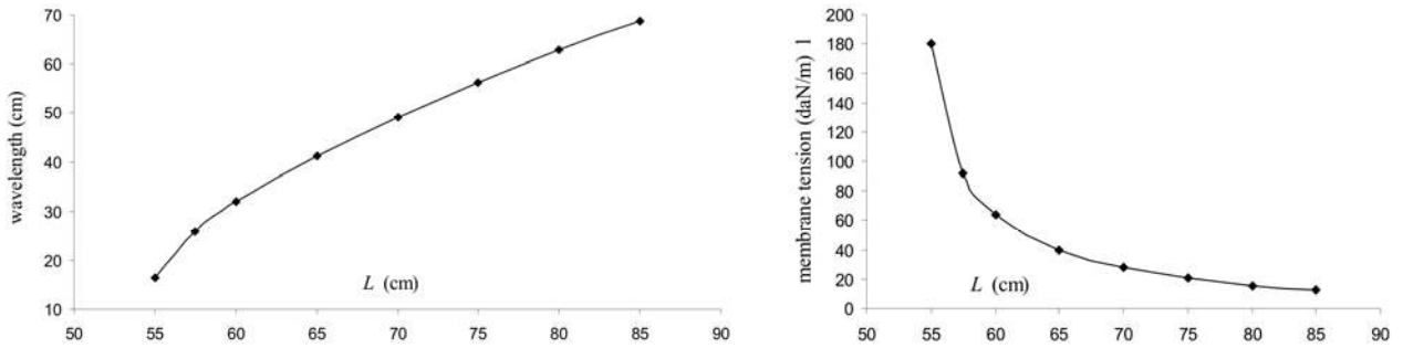
Figure 11. Curves \ell(L) and T_m(L)
