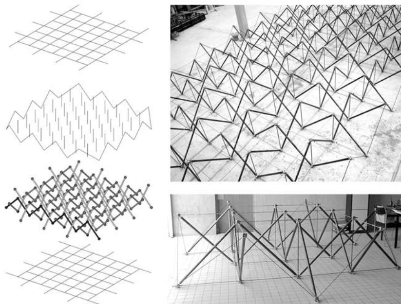
Figure 3. Woven tensegrity grid (Tensarch project)
