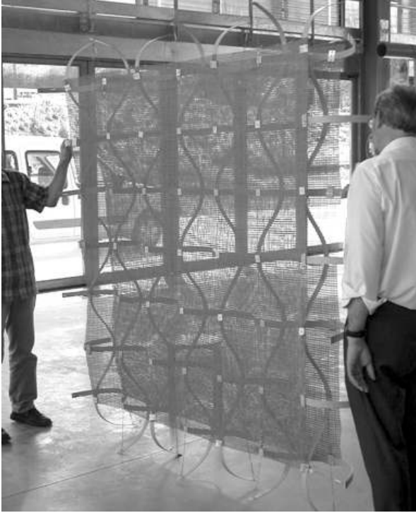
Figure 4. Soft “tensegrity like” panel (external view)
