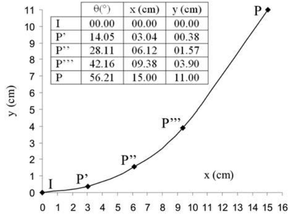
Figure 18. Shape of the strip wave segment (part IP)
