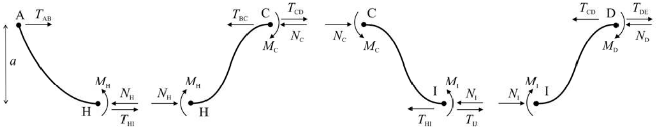
Figure 7. Actions on the different segments of one half strip
