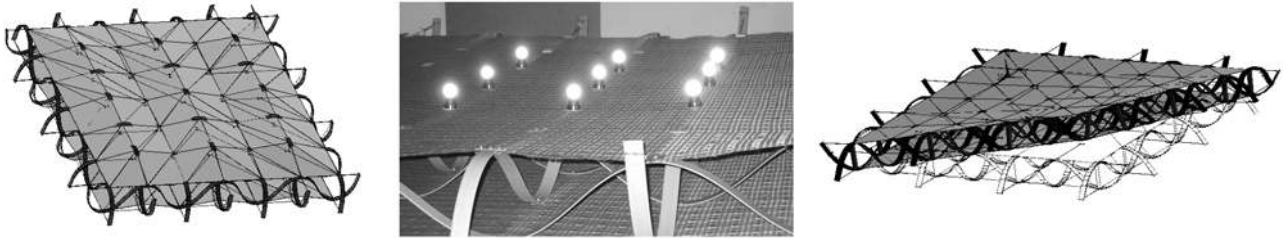
Figure 19. FEM analysis, experimental testing and anticlastic panel generation
