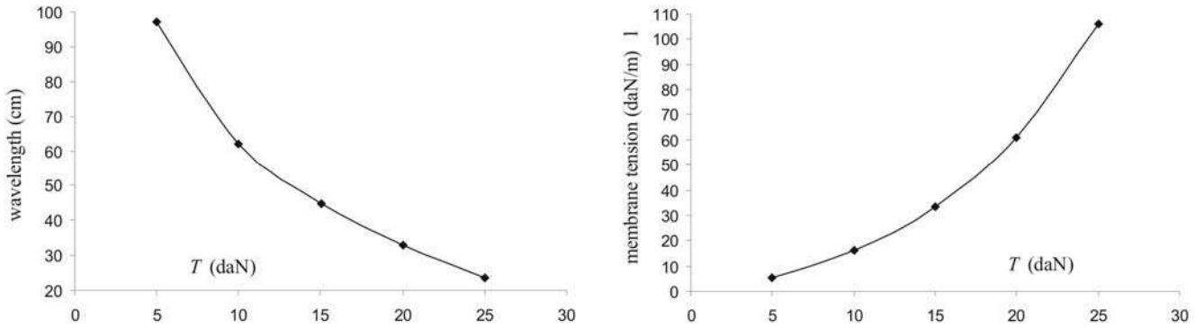
Figure 13. Curves \ell(T) and T_m(T)
