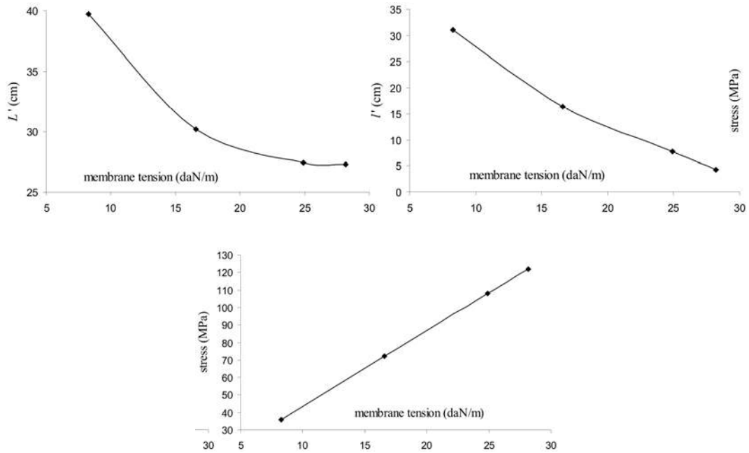
Figure 17. Curves L'(T_m) , \ell'(T_m) and \sigma'_{\max}(T_m) for a strip boundary wave
