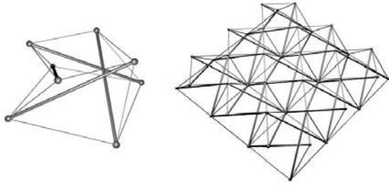
Figure 2. Tensegrity grid composed of identical modules
