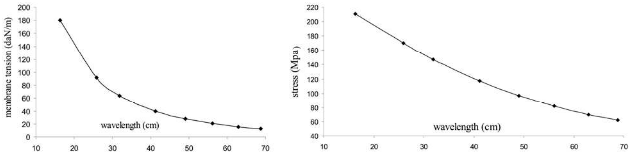
Figure 12. Form control strategy: curves T_m(\ell) and \sigma_{\max}(\ell)
