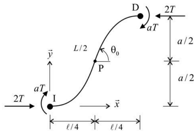
Figure 9. Half-wave segment of the strip
