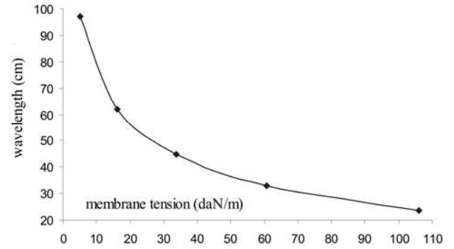
Figure 14. Force control strategy: curve \ell(T_m)
