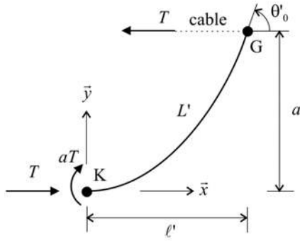
Figure 16. Strip boundary wave
