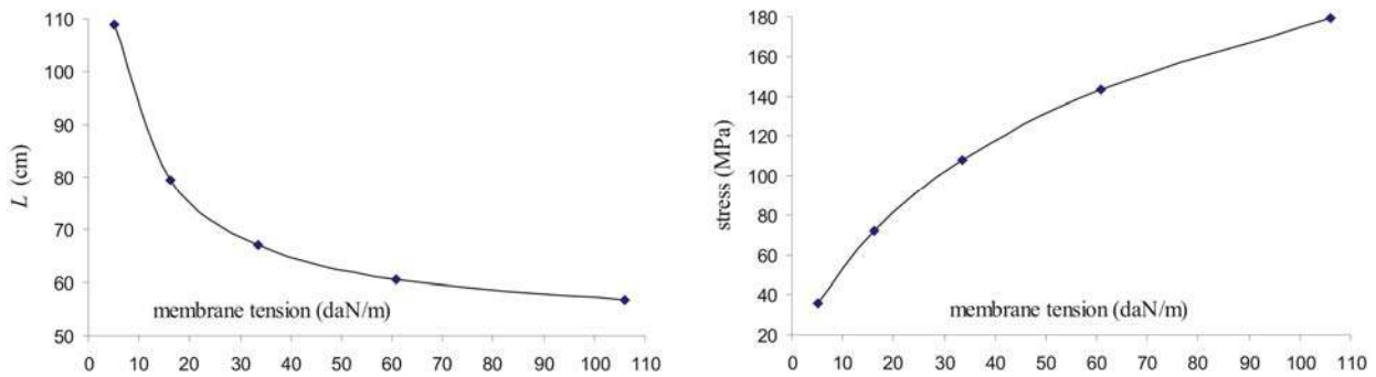
Figure 15: Force control strategy: curves L(T_m) and \sigma_{\max}(T_m)
