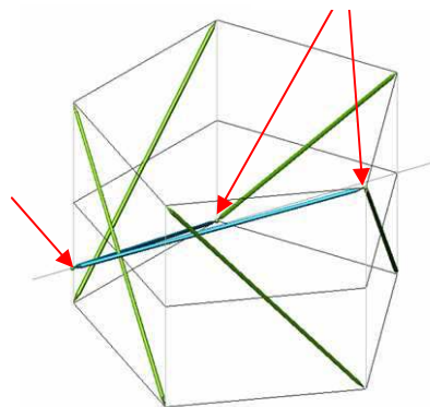
Figure 18. Addition of two supplementary struts
