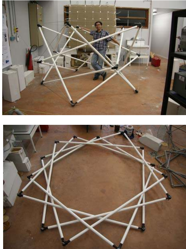
Figure 25. Physical model for a tensegrity ring
