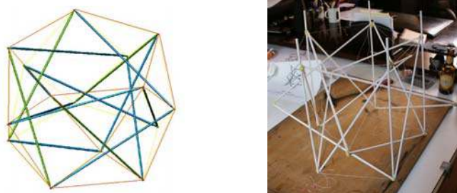
Figure 16. Module assembly
