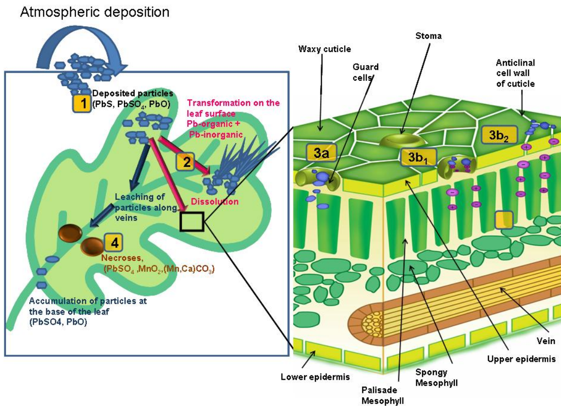
Figure 3. Tentative pathways for lead uptake after deposition of Pb-containing particles. Deposition of particles on the leaf surface (1), chemical transformation on the leaf surface leading to secondary Pb-containing phases and possibly solutes (2). Accumulation of particles in stomata and possibly penetration of nanoparticles (3a). Possible diffusion of solutes via aqueous pores present on cuticular ledges of stomata (3b 1 ) and anticlinal cell walls of cuticles (3b 2 ). Toxicity symptoms (necroses) induced by the presence of the contaminated particles on the leaf (4).
