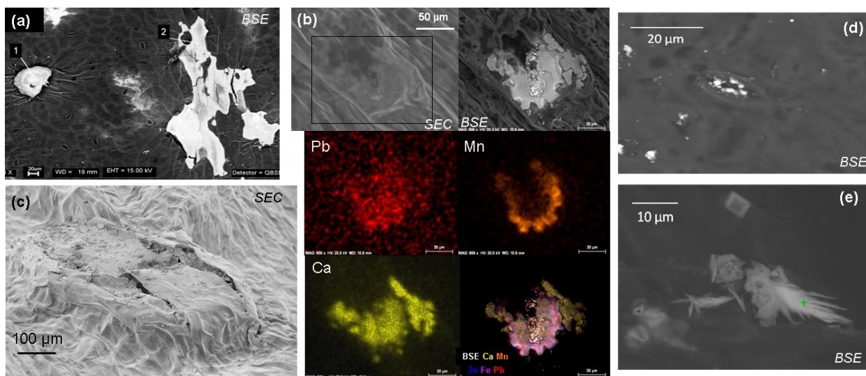
Figure 2 . ESEM-EDX analyses of Pb-rich regions on lettuce leaves exposed to atmospheric fallouts. (a) Two large necroses shown in BSE mode. The EDX semi-quantification for spots 1 and 2 gave 9% Pb, 1% Cl, 1% Mn, 1% Fe, 20% O, 2% Mg and 65% P. (b) SE and BSE images of a necrosis, elemental distribution of Pb, Ca and Mn, and multi-color map showing the distribution of Ca, Mn, Zn, Fe and Mn. (c) SE image of a necrosis. Particles are visible on the leaf surface, as well as beneath the surface. (d) Stomata plugged by Pb-containing particles (e) Secondary Pb-containing compounds formed on the leaf surface.
