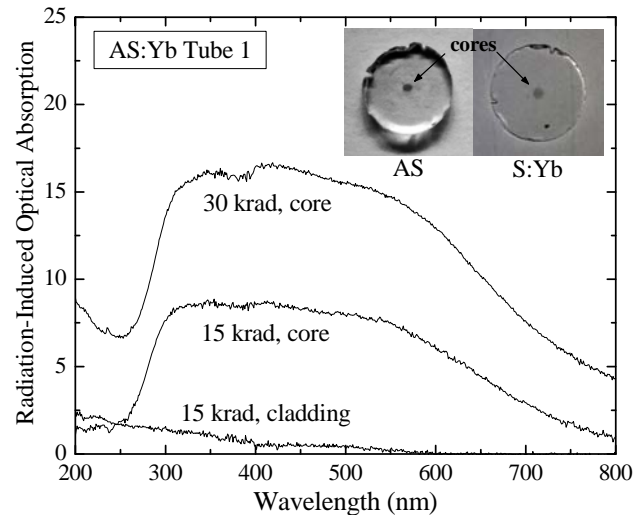
Fig. 2. Radiation-induced optical absorption (RIOA) in the core and cladding of the AS:Yb preform sample made from tube 1. The vertical scale gives the difference, in points, between the optical transmission (in %) before and after irradiation. Insets: photographs of the AS and S:Yb preform samples after X irradiation (dose \sim 50 krad( \text{SiO}_2 )).
