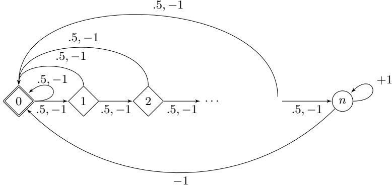
Fig. 1. Player 0 wins in \mathcal{M} if she visits state 0 infinitely many times and she satisfies the \text{Avg}_{>0} objective.
