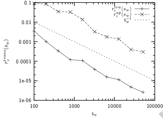
Figure 26: Finite size scaling of the upper and lower transition points r_e^{up} and r_e^{low} , i.e. the points where \alpha^* crosses \alpha_{low}^* and \alpha_{up}^* , respectively (Fig. 25), as a function of the sampling window length s_w . Both r_e^{up} and r_e^{low} vanish \propto s_w^{-1} , as indicated by the line with slope -1 in this log-log-plot.
