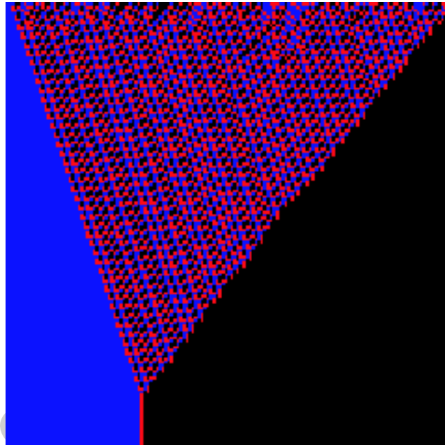
Figure 4: A typical dynamical run for the automata as defined in Table I, here for a system of size N_C = 250 cells (deterministic dynamics, no noise), starting from a random initial configuration. Time is running on the y -axis from top to bottom. Cells with state \sigma_i = 0 are depicted in black color, cells with \sigma_i = 1 in red and cells with \sigma_i = 2 in blue.
