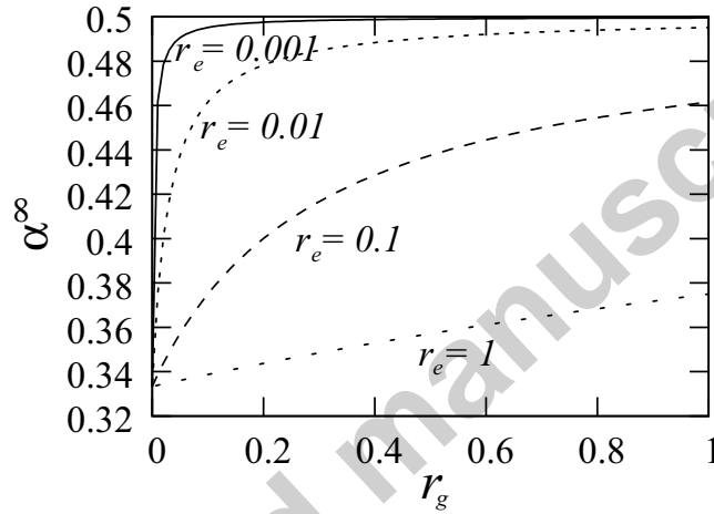
Figure 16: Asymptotic boundary position \alpha^\infty(r_g) in the case of unlimited symmetric growth at the boundaries of the cellular array, for four different error rates r_e .
