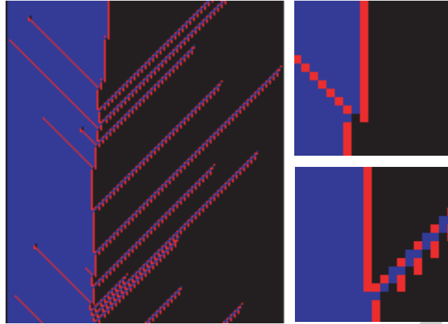
Figure 10: Quasi-particles, started by stochastic update errors, lead to control of the boundary position under noise (left panel). The \Gamma particle (top right) leads to readjustment of the boundary two cells to the left, the \Delta particle (bottom right) leads to readjustment of the boundary one cell to the right.
