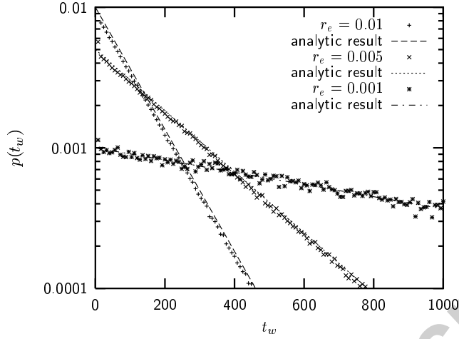
Figure 14: Probability distribution p(t) of waiting times for boundary readjustments in the model with stochastic update errors for three different values of r_e , semi-log plot. As expected for a Poisson process, p(t) is an exponential.
