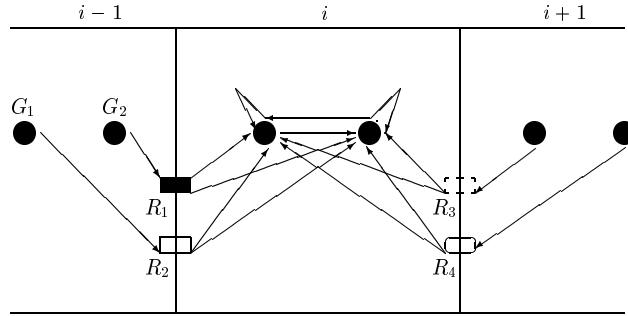
Figure 2: Diagram showing the interaction structure of the minimal network needed to solve the asymmetric expression task. For the sake of clarity, intracellular interactions between the two genes G_1 and G_2 are shown only for cell i , and likewise outgoing intercellular signals from the two genes to the neighbor cells i - 1 and i + 1 were left out. The transcription factors produced by gene G_1 and G_2 in cell i - 1 couple to the receptor systems R_1 and R_2 , respectively, whereas in cell i + 1 the transcription factors produced by these genes couple to the receptor systems R_3 and R_4 (biased signaling). In cell i , the receptors release factors which regulate the activity of G_1 and G_2 .
