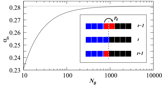
Figure 17: Asymptotic domain boundary position \alpha_\infty (lined curve) as a function of the initial system size N_0 , for homogeneous growth, as explained in the text. One has \alpha_\infty = \alpha_0 - 1/N_0 , where \alpha_0 = 0.281 is the boundary position of the constant-size system (dashed line). Inset : Proliferation of the boundary cell (red) at time t - 1 leads to readjustment of the boundary at its original position (indicated by the dashed line) at time t + 1 , thereby increasing the black domain by one cell and hence slightly reducing \alpha .
