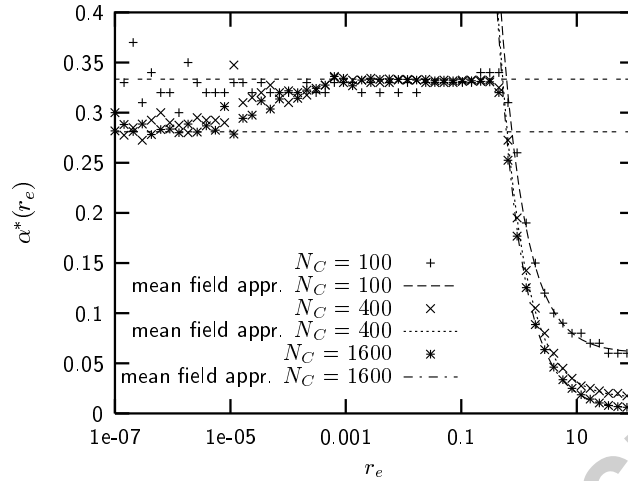
Figure 12: Average boundary position \alpha^* as a function of the error rate r_e for system sizes N_C = 100 , N_C = 400 , and N_C = 1600 . The abscissa is logarithmic. Numerical data are averaged over 200 different initial conditions with 2 \cdot 10^6 updates each. The dashed curves show the mean field approximation given by Eqn. (35), the straight dashed lines mark the unperturbed solution \alpha^* = 0.281 and the solution under noise, \alpha^* = 1/3 .
