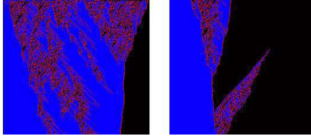
Figure 19: Dynamics of pattern formation under noisy direction recognition; parameters in the simulation shown here were p_{dir} = 0.1 and r_e = 0.003 . Initial pattern formation (left panel) as well as control of the boundary by quasi-particles (right panel) still work, though particle trajectories become broadened and blurred.
