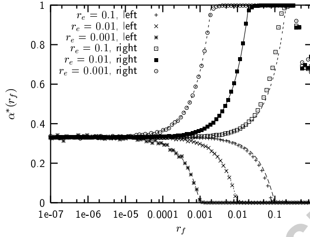
Figure 15: Average domain size \alpha^* as a function of the the cell flow rate r_f for three different error rates r_e ; numerical data (crosses and points) were sampled over 10 different initial conditions and 10^6 updates for each data point. “Left” indicates cell flow directed to the left system boundary, “right” to the right system boundary, respectively. The dashed lines are the corresponding solutions of Eqn. (25).
