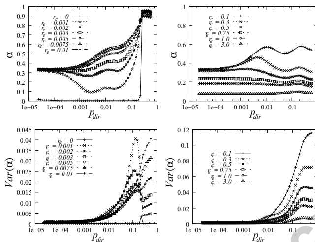
Figure 20: Upper panels : average boundary position \alpha as a function of p_{dir} , for different values of r_e . Left panel: low noise limit ( r_e \rightarrow 0 ), right panel: high noise limit. Lower panels : Fluctuations (temporal variance) of the boundary position as a function of p_{dir} .
