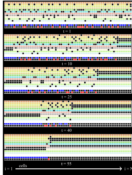
Figure 9: Snapshots of spatial gene activity patterns of the network shown in Fig. 6., for a system of 80 coupled networks (cells) at different update times t . Each row shows the state of one network gene, color coding is the same as in Fig. 8; if the respective gene is not active in the cell at time t , the cell is shown in black color. The two bottom rows show the states of the two target (pattern) genes. After 55 update time steps, the target pattern (compare Fig. 4) has self-organized.
