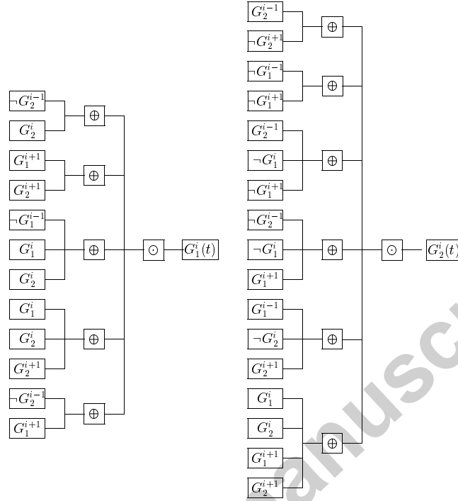
Figure 7: Boolean representation of the minimal network, minimized conjunctive normal form. G_a^b with a \in \{1, 2\} and b \in \{i-1, i, i+1\} denotes gene a in cell number b . The inputs in the left branches of the trees are given by the genes' states at time t-1 . \neg denotes NOT, \odot denotes logical AND and \oplus logical OR.
