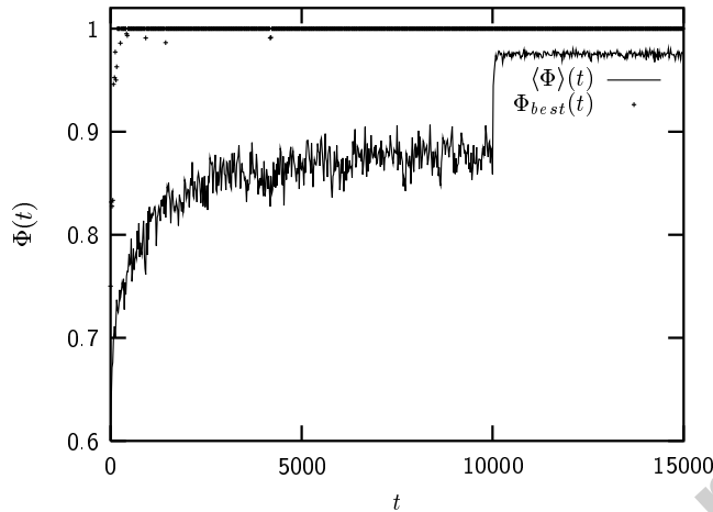
Figure 21: Average fitness \langle \Phi \rangle(t) of the mutant population \mathcal{F}^* and fitness of the highest fitness mutant \Phi_{best}(t) as a function of simulation time during the genetic algorithm run that lead to the high fitness solution used in this paper. At time step 10000 mutations were turned off, in order to test the established population of optimized rule tables under different initial conditions (this corresponds to the sharp increase of \langle \Phi \rangle(t) at time step 10000). The evolved population of rule tables has an average fitness of about 0.98, independent from the initial conditions and system size N_C (in the tested range, i.e. 15 \leq N_C \leq 150 ).
