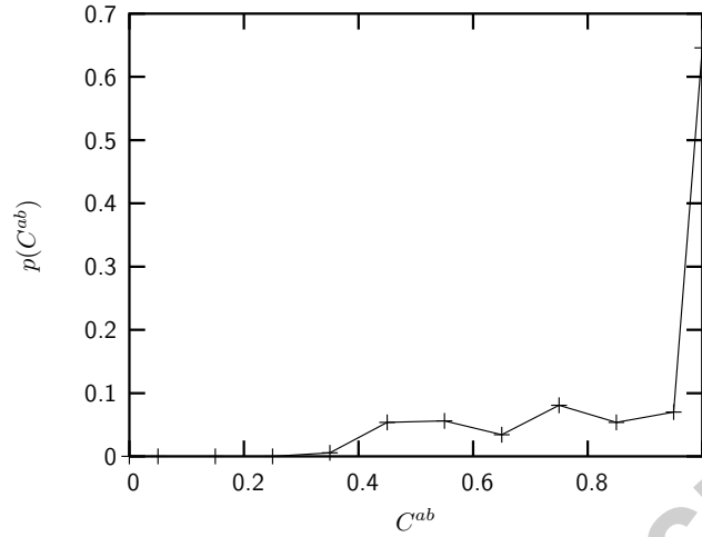
Figure 24: Frequency distribution p(C^{ab}) of two point correlations C^{ab}(\sigma, \sigma') of rule table entries, as defined in Eqn. (B2), averaged over all possible pairs of rule table entries. About 65% of rule table entries have correlation 1.0, for the rest the correlation is lower.
