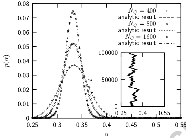
Figure 13: For the system with stochastic update errors, fluctuations of the boundary position \alpha around the average position \alpha^* = 1/3 are Gaussian distributed. The figure compares the numerically obtained stationary probability distribution with the analytic result of Eqn. (23) for three different system sizes. All data are gained for r_e = 0.1 and averaged over 100 different initial conditions with 2 \cdot 10^6 updates each. The inset shows a typical timeseries of the boundary position.
