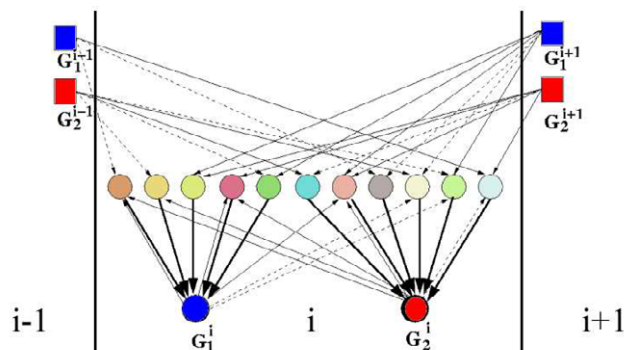
Figure 8: Threshold network realization of the pattern formation system. Solid line arrows denote links with w_{ij} = +1 , dashed arrows denote links with w_{ij} = -1 . The inputs from the genes in the neighbor cells ( G_1^{i-1}, G_2^{i-1}, G_1^{i+1} and G_2^{i+1} ) are processed by a layer of “hidden genes” (colored circles in the middle of the scheme) with different thresholds h implementing a logical OR operation on the inputs. The processed signals then are propagated to the two pattern genes G_1 and G_2 . The threshold of gene G_1 is h_1 = -5 , for gene G_2 one has h_2 = -6 (logical AND). Notice several feed-back connections from genes G_1^i and G_2^i to the hidden layer.
