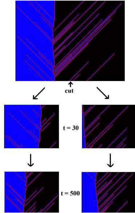
Figure 18: A simulated cut experiment. After 300 updates, a system of 500 cells was cut into two sub-systems of 250 cells each (upper panel). After only 30 updates, in both sub-systems reorganization of the boundary position starts (middle panels). After about 500 system updates, both sub-systems have self-organized into the target pattern with \alpha = 1/3 (bottom panels). In the simulation, r_e = 0.01 was applied.
