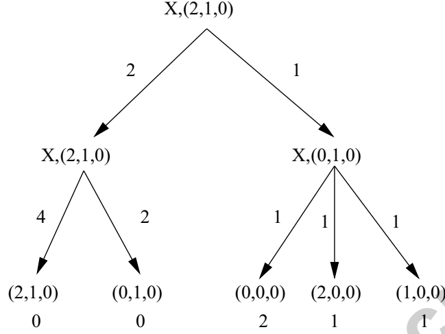
Figure 6: Transition tree for the boundary configuration (2,1,0) . Depending on the state of the left cell X , transition to different configurations occur. Numbers on arrows indicate the total number of the respective branches, the numbers at the bottom are the velocity (boundary readjustment) contributions of the respective branches. For details, see text.
