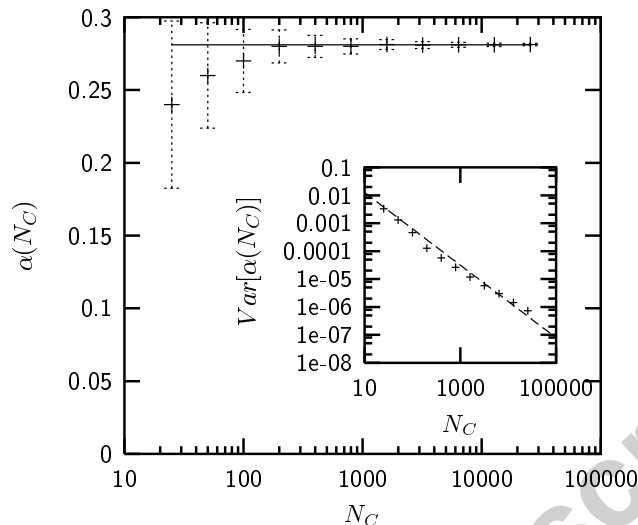
Figure 5: Finite size scaling of the self-organized relative domain size \alpha as a function of the total number of cells N_C . In the limit of large system sizes, \alpha converges towards a fixed value \alpha_\infty = 0.281 \pm 0.001 (as denoted by the straight line fit). The inset shows the finite size scaling of the variance Var[\alpha(N_C)] ; the straight line in this log-log plot has slope -1.3 and indicates that fluctuations vanish with a power of the system size.
