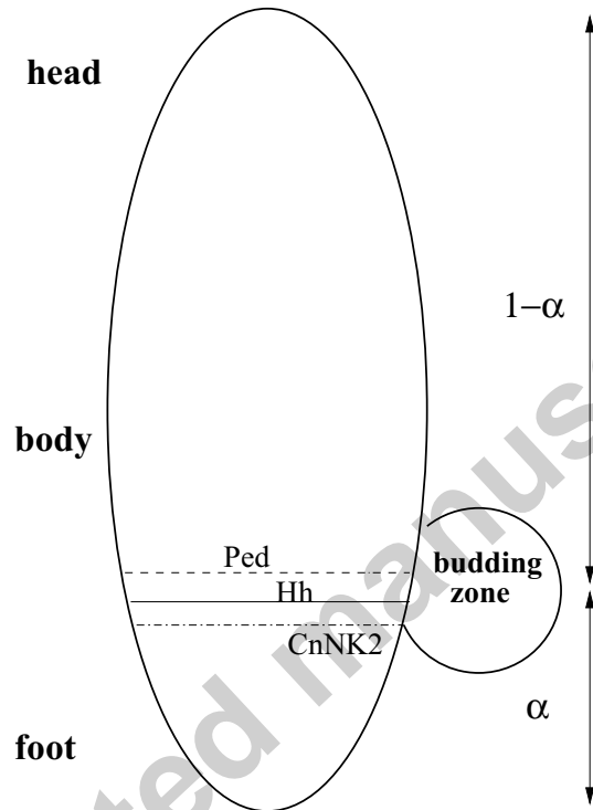
Figure 1: Gene expression domains in Hydra , here for the example of the “foot” genes Pedibin (Ped) and Cn-NK2, and Hedgehog (Hh). Ped and Hh expression are bounded towards the body region of the animal; while Ped exhibits a graded decay in the budding region, Hh exhibits a sharp boundary. The relative position of the budding region and the associated expression boundaries, given by the ratio \alpha/(1 - \alpha) , is independent of the absolute size of the animal (proportion regulation). Details are explained in the text.
