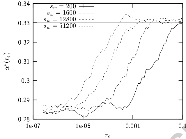
Figure 25: Average domain boundary position \alpha^* as a function of the error rate r_e , sampled over update windows of different lengths s_w (ensemble statistics, 400 different initial conditions for each data point). The abscissa is logarithmic. With increasing s_w , the transition from the solution \alpha_{det}^* = 0.281 under deterministic dynamics to \alpha^* = 1/3 under noise is shifted towards r_e = 0 . The two straight lines define a lower boundary \alpha_{low}^* and an upper boundary \alpha_{up}^* , as explained in the text.
