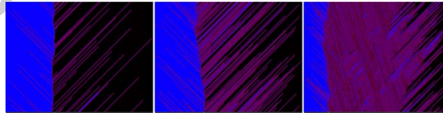
Figure 11: For moderate error rates r_e , the domain boundary is stabilized at an average position \alpha^* = 1/3 (left panel, r_e = 0.1 ). Around r_e \approx 0.2 , there is a crossover to a domain size vanishing with r_e^{-1} (middle panel). In the right panel, the high noise limit is shown, with a considerably shrunk blue domain due to strong particle interference ( r_e = 2.0 ).
