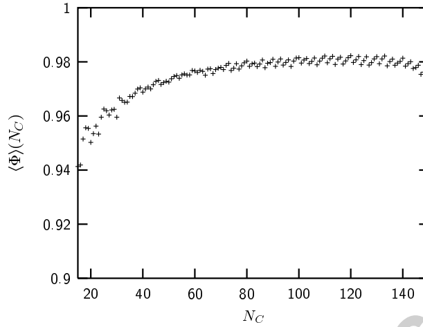
Figure 22: Average fitness of the highest fitness rule table as a function of the system size N_C . For system sizes N_C \geq 80 the fitness is almost constant at about 0.98. Notice that the decrease of the fitness for small N_C is an effect of the dynamics , not of the genetic algorithm implementation (all N_C in the range 15 \leq N_C \leq 150 were tested with equal probability), hence the dynamics of pattern formation may impose a lower boundary on the range of system (animal) sizes tolerated by natural selection.
