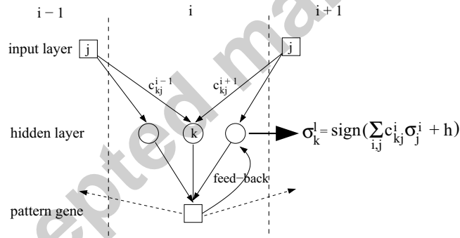
Figure 3: Schematic sketch of a threshold network controlling spatial gene activity patterns. Signals from genes in direct neighbor cells constitute the input layer of the network. In the hidden layer , this information is processed, with logical functions implemented as weighted sums of the inputs. The output of the genes in this layer then controls the pattern genes . Notice that there is feed-back to the hidden layer, as well as to the neighbor cells (dashed arrows).
