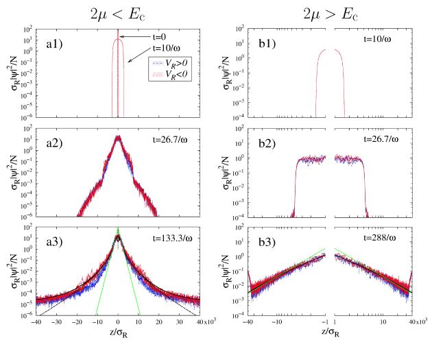
Figure 1. (color online) Time evolution of the density profile of a matter wave expanding in 1D speckle potentials for 2\mu < E_c (left panel) and 2\mu > E_c (right panel). Shown are the running averages, \tilde{n}(z) = \int_{-l/2}^{+l/2} \frac{dx}{l} n(z+x) with l = 100\sigma_R , of numerical data, for blue- and red-detuned speckle potentials (three realizations each) [23]. Here, we use \omega = 2 \times 10^{-2} \mu/\hbar and V_R = \pm 0.0325E_c . Left panel [(a1)-(a3)]: semi-logarithmic scale for \xi_{in} = 1.5\sigma_R ( 2\mu \simeq 0.44E_c ). The solid black line shows a fit of the full Eq. (5) and the dotted black line to Eq. (5) with A(p, E) \rightarrow \delta(E - p^2/2m) , both with a multiplying factor as the only fitting parameter. The dashed green line is a fit of \ln[n(z)] = A - 2\gamma(2\mu)|z| , with A as the fitting parameter. Right panel [(b1)-(b3)]: log-log scale for \xi_{in} = 0.83\sigma_R ( 2\mu \simeq 1.44E_c ). The solid black line shows the full Eq. (5) and the dashed green line is a fit of n(z) = A/|z|^\beta with A and \beta as the fitting parameters.
