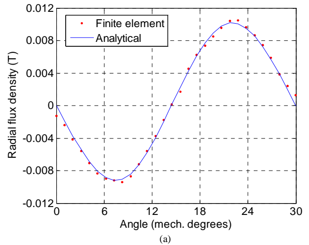
Fig. 14. Flux density distribution for radial (a) and tangential (b) component of armature reaction field in the middle of the airgap domain: J_{ms}=4.6A/mm^2 , I_a = I and I_b = I_c = -I/2 , and \beta/\delta = 0.4 .
