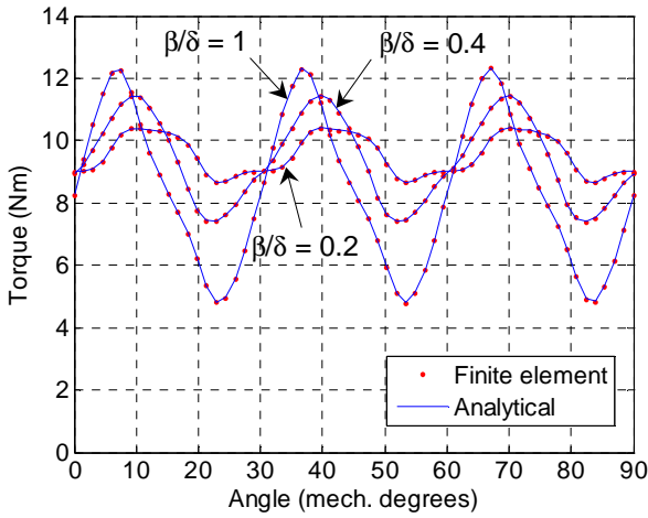
Fig. 20. Electromagnetic torque versus rotor position for different values of \beta/\delta ( J_{rms}=4.6A/mm^2 )
