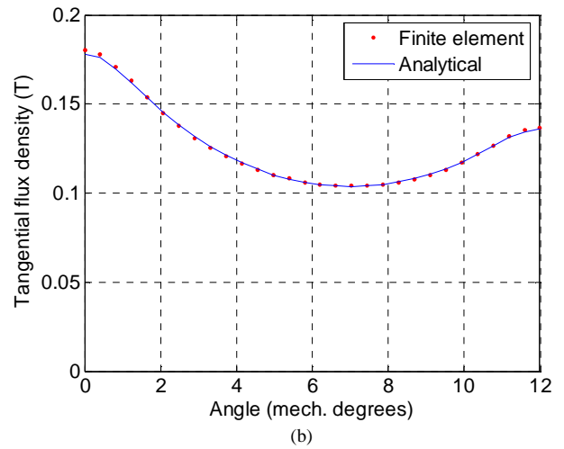
Fig. 15. Flux density distribution for radial (a) and tangential (b) component of armature reaction in the middle of the slot-opening domain for \beta/\delta = 0.4 .
