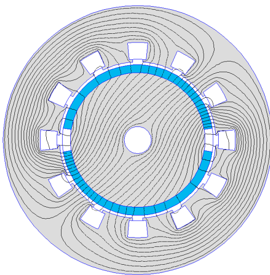
Fig. 24. Magnetic flux lines under load condition ( \beta/\delta = 0.6 )
