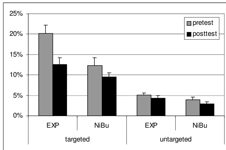
Figure.5. Mean error percentages (and SEMs) for errors on the targeted and untargeted phonemes.
