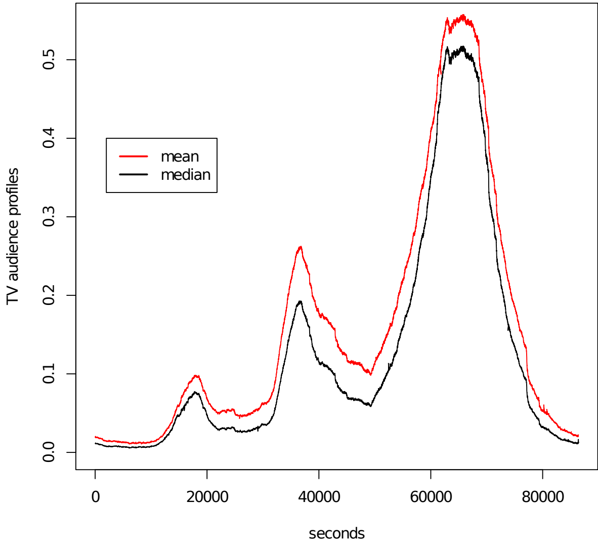
Figure 1: Estimations of the mean and the geometric median audiences, at a second scale, during the 6th september 2010.
