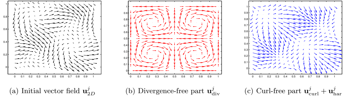
Figure 5. Example of Helmholtz decomposition.
