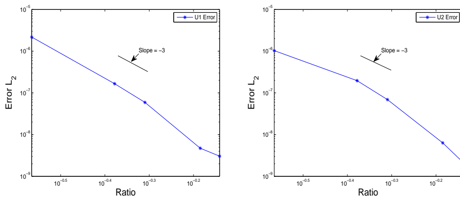
FIGURE 10. Error on the first component \mathbf{u}_1 (left) and on the second component \mathbf{u}_2 (right), provided by the nonlinear approximation of \mathbf{u} in \mathbb{V}_j^{div} , versus the ratio of retained coefficients (log-log scale).
