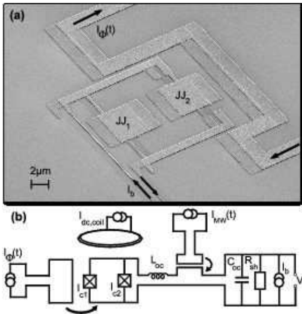
FIG. 4: (a) SEM image of a Camelback phase qubit based on a dc SQUID after lift-off.(b) The dc SQUID phase qubit is controlled by a dc bias current I_b and flux \Phi_b , manipulated by a MW current and measured by a nanosecond flux pulse. The qubit is decoupled from the environment by a large kinetic inductance L_e = 10nF and capacitance C_e = 200pF and is shunted by a resistance R_{sh} = 20k\Omega .
