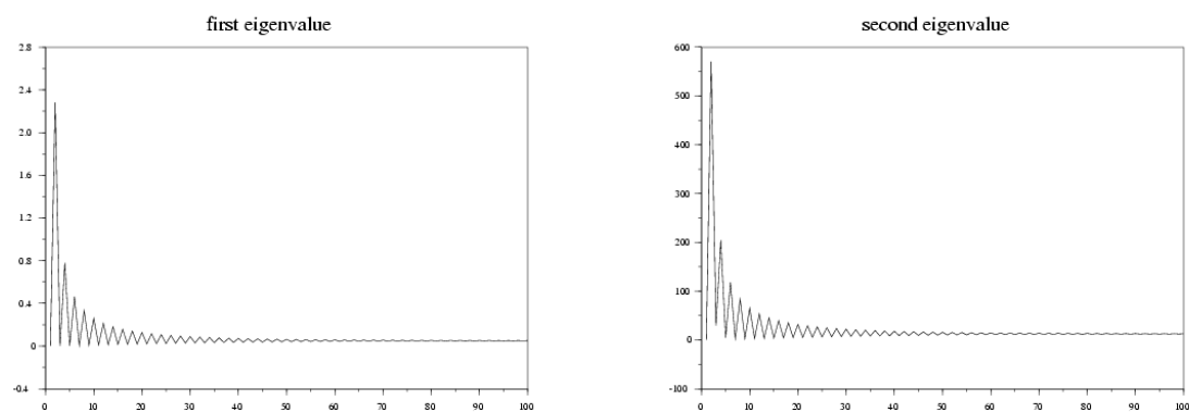
Figures 11 and 12. Harmonic oscillator.
