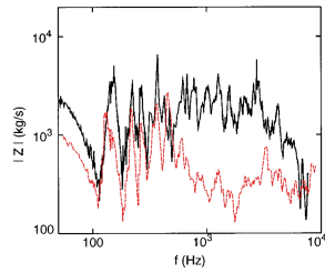
Figure 3: Comparison of the driving point impedance measured on an upright piano in two different locations. —: at bridge (terminating point for strings of C_4 – key n° 40), after Giordano (1998). - - -: far away from the bridge, at a mid-point between two ribs.
