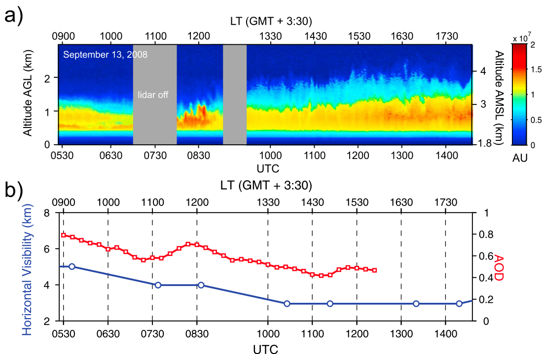
Figure 6. (a) Time-height series of lidar attenuated backscatter profiles recorded in Zanjan (at 532 nm) between 0530 UTC and 1430 UTC on 13 September 2008. Both UTC time (bottom axis) and local time (top axis) as well as both altitude above ground level (left axis) and above sea level (right axis) are indicated. (b) AOD measured by the SPM in Zanjan between 0525 UTC and 1230 UTC at 670 nm (the SPM stopped working after 1230 UTC) and horizontal visibility reported by the Zanjan meteorological station ground observer between 0520 UTC and 1500 UTC on 13 September 2008.
