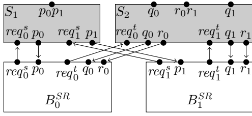
Figure 9. A Send/Receive composite component with Decentralized Scheduler
