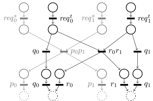
Figure 8. Splitting the scheduler
