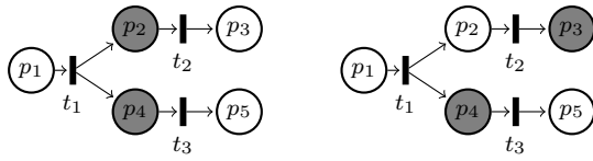
Figure 5. An example of a simple Petri net
