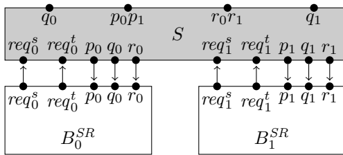
Figure 7. A composite Send/Receive component
