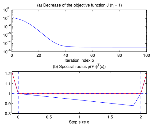
Fig. 3. Unsupervised NMF
