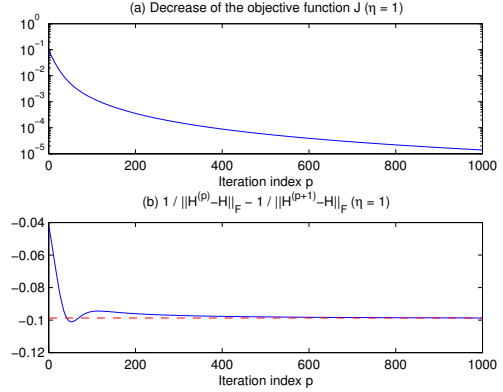
Fig. 1. Example of sub-linear convergence speed
