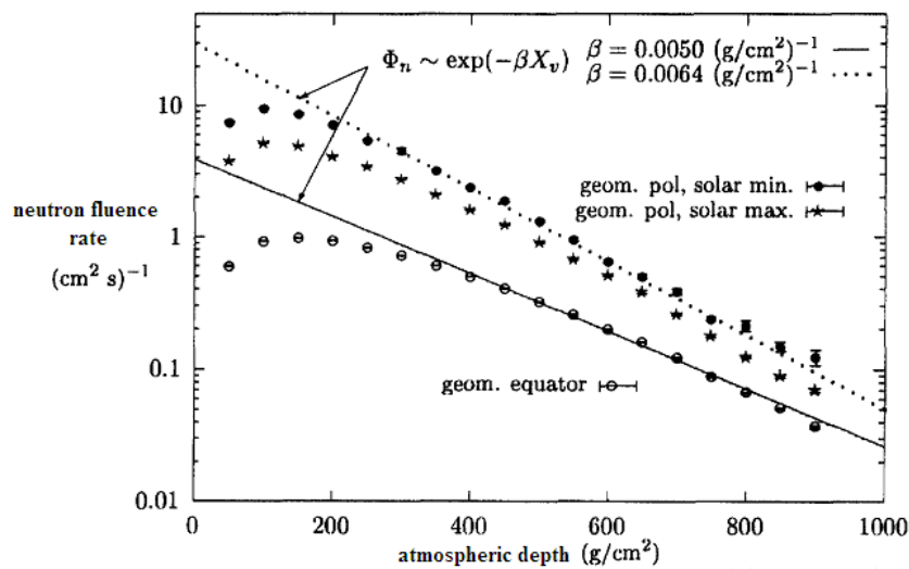
Figure 3: the depth dependence of the neutron flux, calculates for three different conditions. Polar region (minimum and maximum) and equatorial region.
