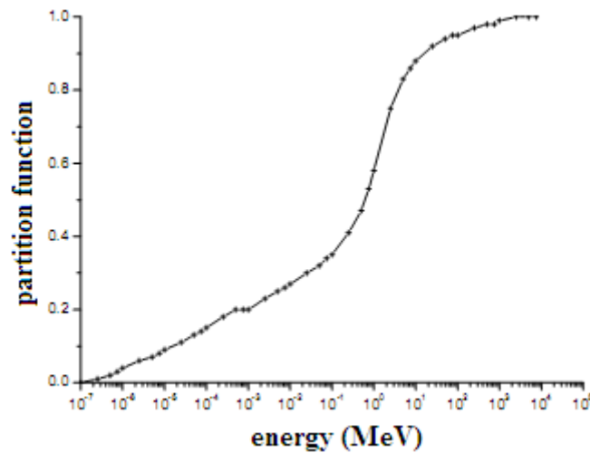
Figure 6: cumulative distribution function related to incident energy neutron
