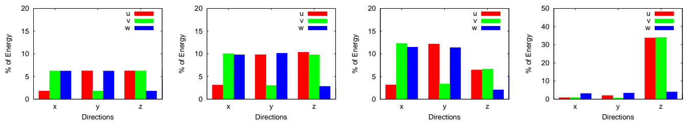
FIG. 5: (Color online) Directional energy of the three velocity components u , v and w for (from left to right) divergence-free Gaussian white noise, isotropic, rotating and stratified turbulence.
