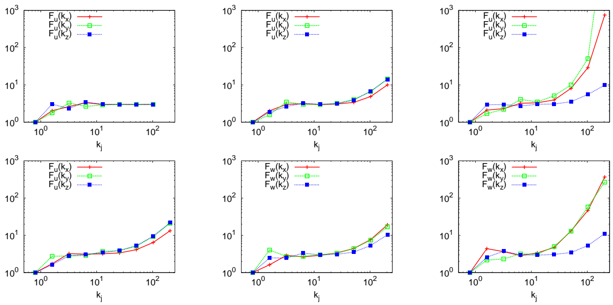
FIG. 6: (Color online) Directional scale-dependent flatness for Gaussian white noise (left top) and isotropic turbulence u component (left bottom), rotating turbulence, u and w components (middle) and stratified turbulence, u and w components (right).
