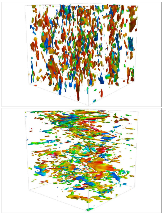
FIG. 1: (Color online) Iso-entrophy surfaces from direct numerical simulation for rotating (top) and stratified (bottom) turbulence with an iso-value equal to the mean entrophy. In the rotating case we observe elongated vertical structures, in the stratified case flattened horizontal structures. The vertical velocity is shown in the visualization by a color scale ranging from blue (negative velocity) to red (positive velocity).
