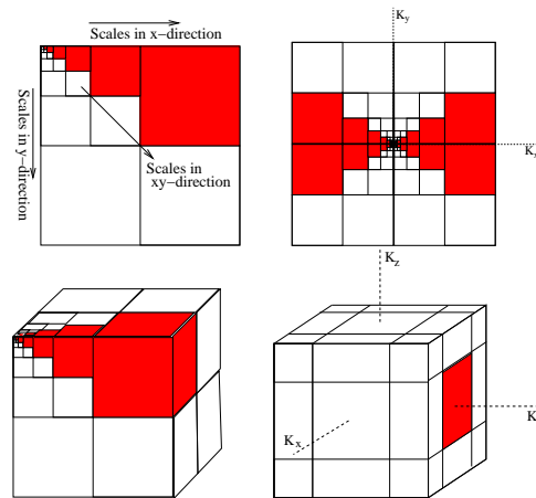
FIG. 2: (Color online) Left: wavelet space in two and three dimensions. Right: wavelet space projected onto Fourier space. Each box corresponds to a certain scale j and direction d and each box contains 2^{2j} values of \mathbf{i} in two dimensions and 2^{3j} in three dimensions, giving information on localization in physical space. Hereby we can relate a scale j to a wavenumber k_j : k_j = k_0 2^j , where k_0 is the centroid-wavenumber of the wavelet.
