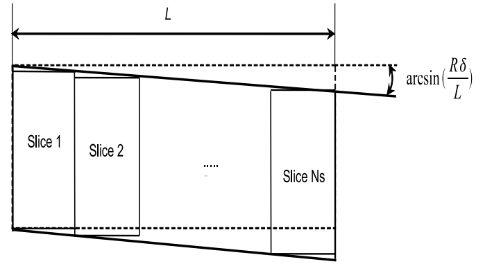
Fig. 2. Axial view of the skewed rotor.
