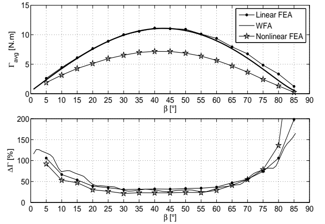
Fig. 10. Average torque and torque ripple vs \beta of the skewed ( \delta = 10^\circ ) machine.
