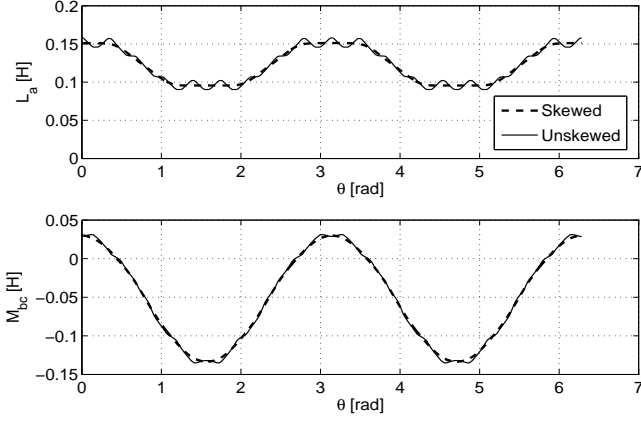
Fig. 3. Self- and mutual- skewed ( \delta = 10^\circ ) inductances, with \beta = 0.5 , e_2 = 10\text{mm} , not chorded winding, skewed rotor.
