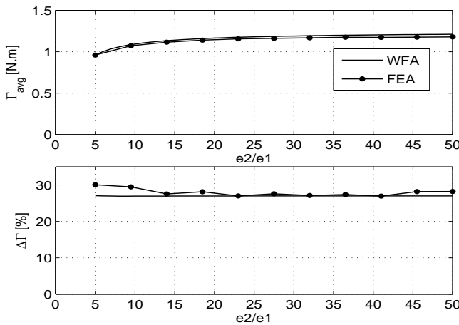
Fig. 9. Average torque and torque ripple vs interpolar gap length e2 to air-gap length e1 ratio of the skewed ( \delta = 10^\circ ) machine.
