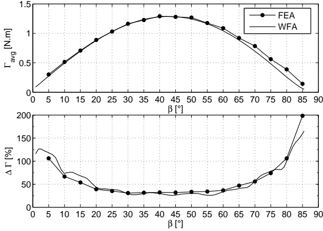
Fig. 8. Average torque and torque ripple vs \beta of the skewed ( \delta = 10^\circ ) machine.
