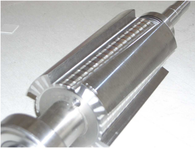
Fig. 11. Photography of the prototype rotor.
