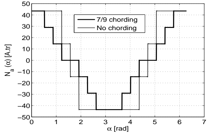
Fig. 6. No chording and \frac{7}{9} chording winding function of the phase "a".
