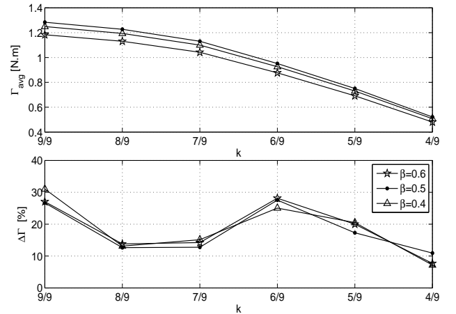
Fig. 7. Average torque and torque ripple vs chording factor of the skewed ( \delta = 10^\circ ) machine.
