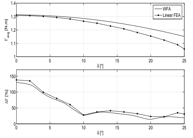
Fig. 5. Average torque and torque ripple vs skewing angle.
