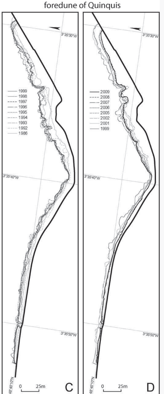
Figure 8 (this and opposite page). Shoreline changes as deduced from measurement of foredune changes at Saint-Efflam (A and B), Quinquis (C and D), Grand Rocher (E and F), Tréduder (G), and Saint-Michel-en-Grève (H and I) between 1986 and 2009.
