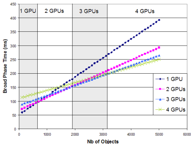
Figure 6: Results of off-line simulations performed on a 4*Quadro FX 5800 platform. We measured time spent by 1, 2, 3 and 4 GPUs in relation to the number of objects in the environment.
