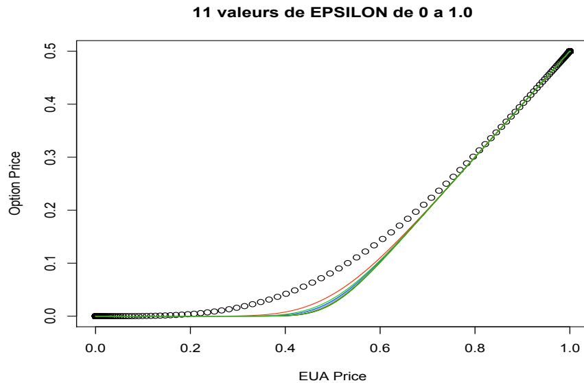
FIGURE 1. European call option prices for \epsilon = 0, 0.1, 0.2, \dots, 0.9, 1 .
