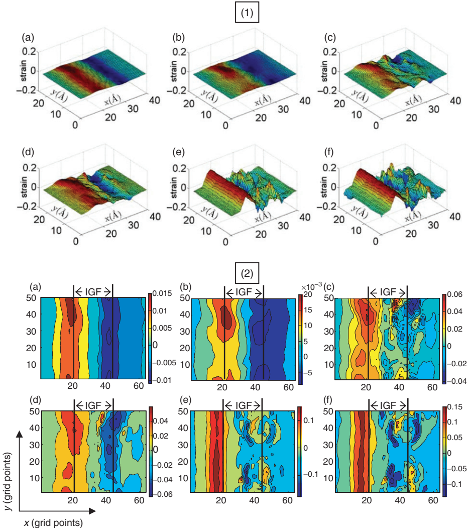
Figure 5. Local axial strains, \epsilon_{xx} , plotted as (1) 3D surface plots and (2) 2D contour plots for x -direction loading at overall strain levels of (a) 0.23%, (b) 0.46%, (c) 0.93%, (d) 1.38%, (e) 1.85%, and (f) 2.31%, showing progressive development of tensile strain band along the interface between the intergranular glassy film (IGF) and crystalline layers, and compressive strain band within the IGF (See online for colour version).
