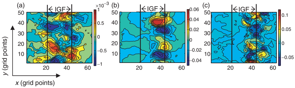
Figure 6. Contours of local lateral strains, \epsilon_{yy} , for x -direction loading at overall strain levels of (a) 0.23%, (b) 0.93% and (c) 1.85% showing periodic compressive and tensile bands within the intergranular glassy film (IGF) (See online for colour version).
