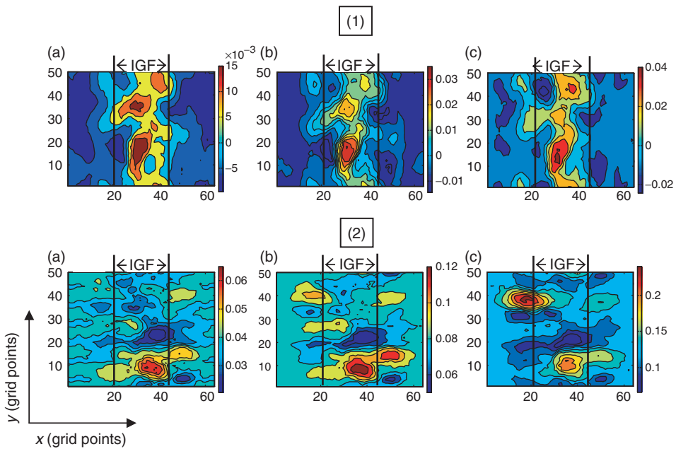
Figure 7. Contours of (1) local lateral strains, \epsilon_{xx} , and (2) local axial strains, \epsilon_{yy} , for y -direction loading at overall strain levels of (a) 4%, (b) 8% and (c) 12% (See online for colour version).
