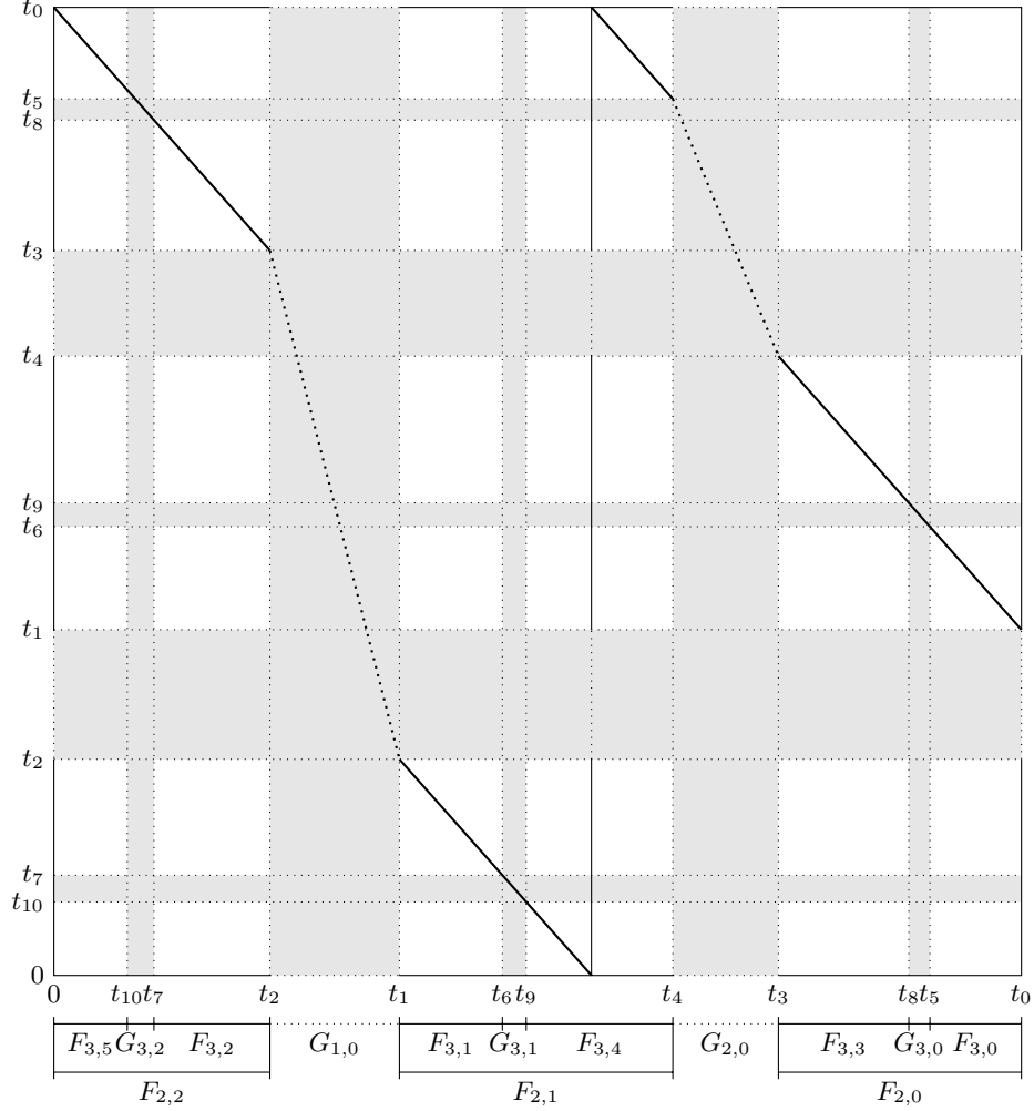
FIGURE 3. The (-\beta) -transformation for \beta = 9/8 with gaps G_{m,k} , support of the invariant measure F_{3,0} \cup \dots \cup F_{3,5} , and t_k = T^k_{-\beta}(1) . Ratios between G_{1,0} , G_{2,0} and the rest of the picture are not respected. In reality, G_{1,0} is almost 10 times the size of G_{2,0} , and G_{2,0} is almost 5 times the size of F_{2,0} .
