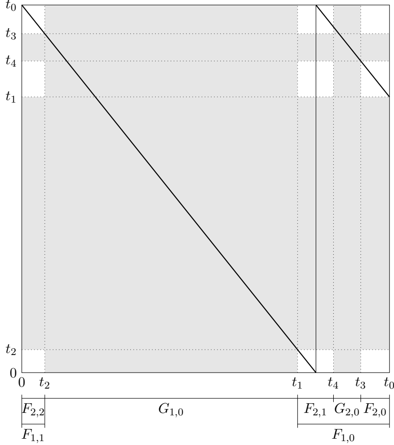
FIGURE 2. The (-\beta) -transformation for \beta = 5/4 , with set of gaps G_{1,0} \cup G_{2,0} and support of the invariant measure F_{2,2} \cup F_{2,1} \cup F_{2,0} . Here, t_k = T^k_{-\beta}(1) .
