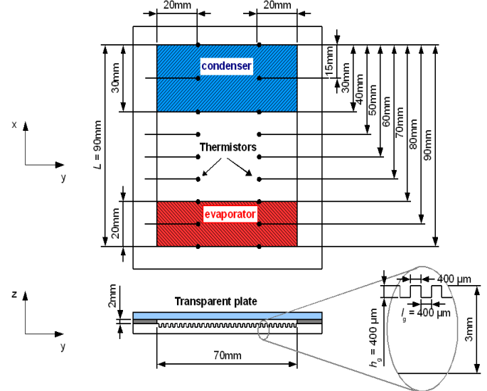
Fig. 4 FPHP made of copper
